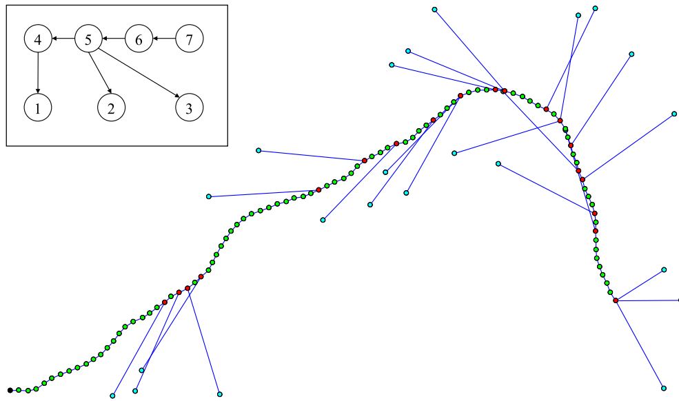
Figure 7: The elimination tree for the LX ordering of Figure 6, showing how the state and landmarks estimates will be computed via back-substitution: the root is computed first - here the first pose on the left - and proceeds down the Markov chain to the right. Landmarks can be computed as soon as the pose they are connected to has been computed.
