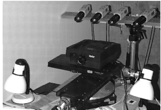
Figure 1. The scanner hardware.
