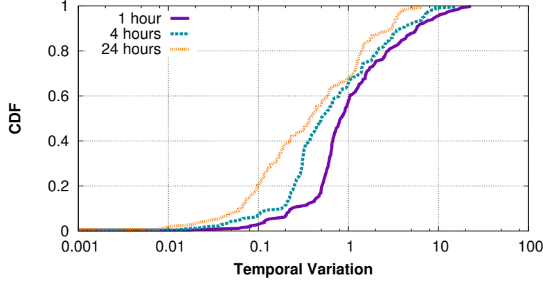
Figure 3-3: Temporal variation in the HPCS dataset.
