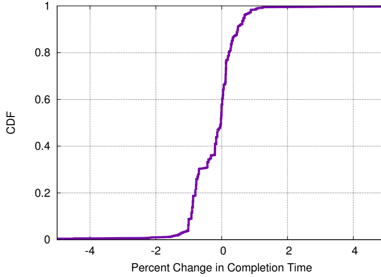
Figure 4-8: Percent change in completion time when measuring the network only once vs. every five minutes.
