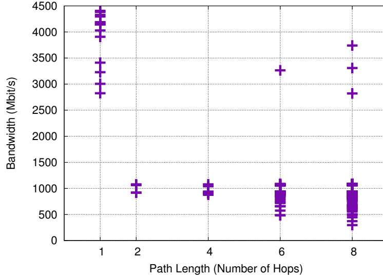
Figure 6-9: Comparison of path length with achievable throughput. Path length is not entirely correlated with throughput, as evidenced by the eight-hop paths with throughput over 2500 Mbit/s.
