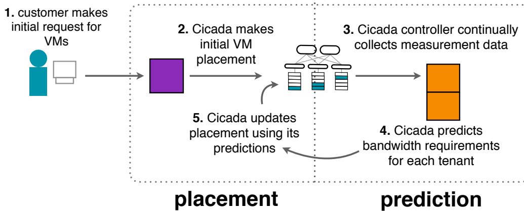
Figure 2-2: Cicada’s architecture.
