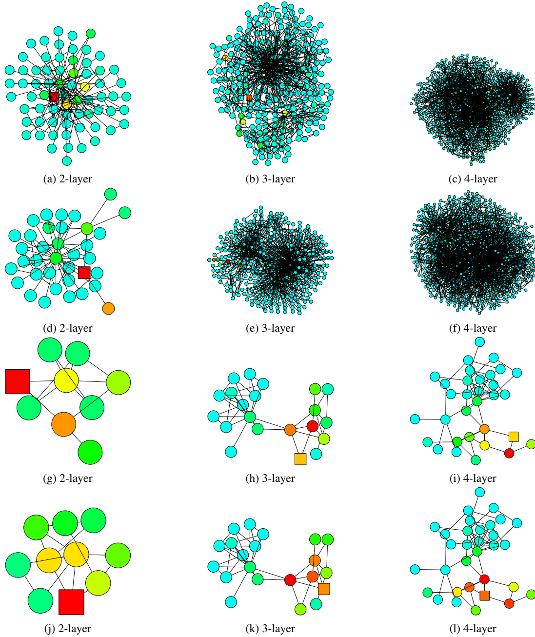
Figure 8. Subgraph structures where 3, 4-layer GCNs make misclassification, whereas 2-layer GCNs make the correct prediction.
