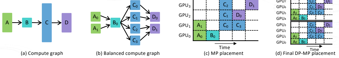
Figure 4: An example of SiP-ML’s parallelization strategy with k = 4 , l = 2 , \mathcal{D}=3 , and \Delta = 2 .
