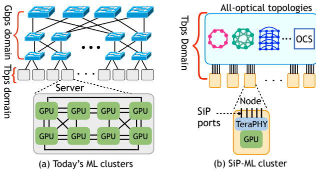
Figure 2: Comparing today’s ML cluster with SiP-ML.
