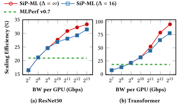
Figure 14: Comparing the scaling efficiency of our placement algorithm at different bandwidths to state-of-the-art expert designed placements in MLPerf benchmark for 1024 GPUs.
