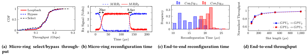
Figure 12: Testbed benchmarks.
