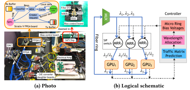
Figure 11: SiP-ML’s testbed.
