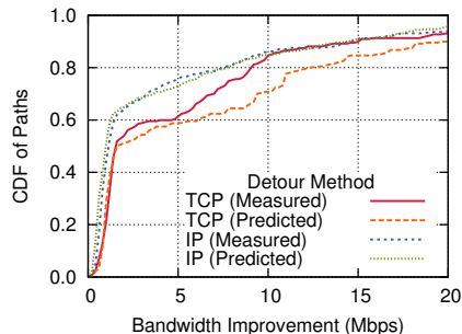
Fig. 4. TCP detouring improves actual bandwidth between nodes significantly more than IP detouring on UkairoLab.
