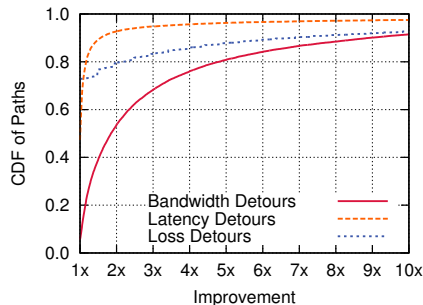
Fig. 3. Bandwidth can be improved significantly more than latency using detouring.
