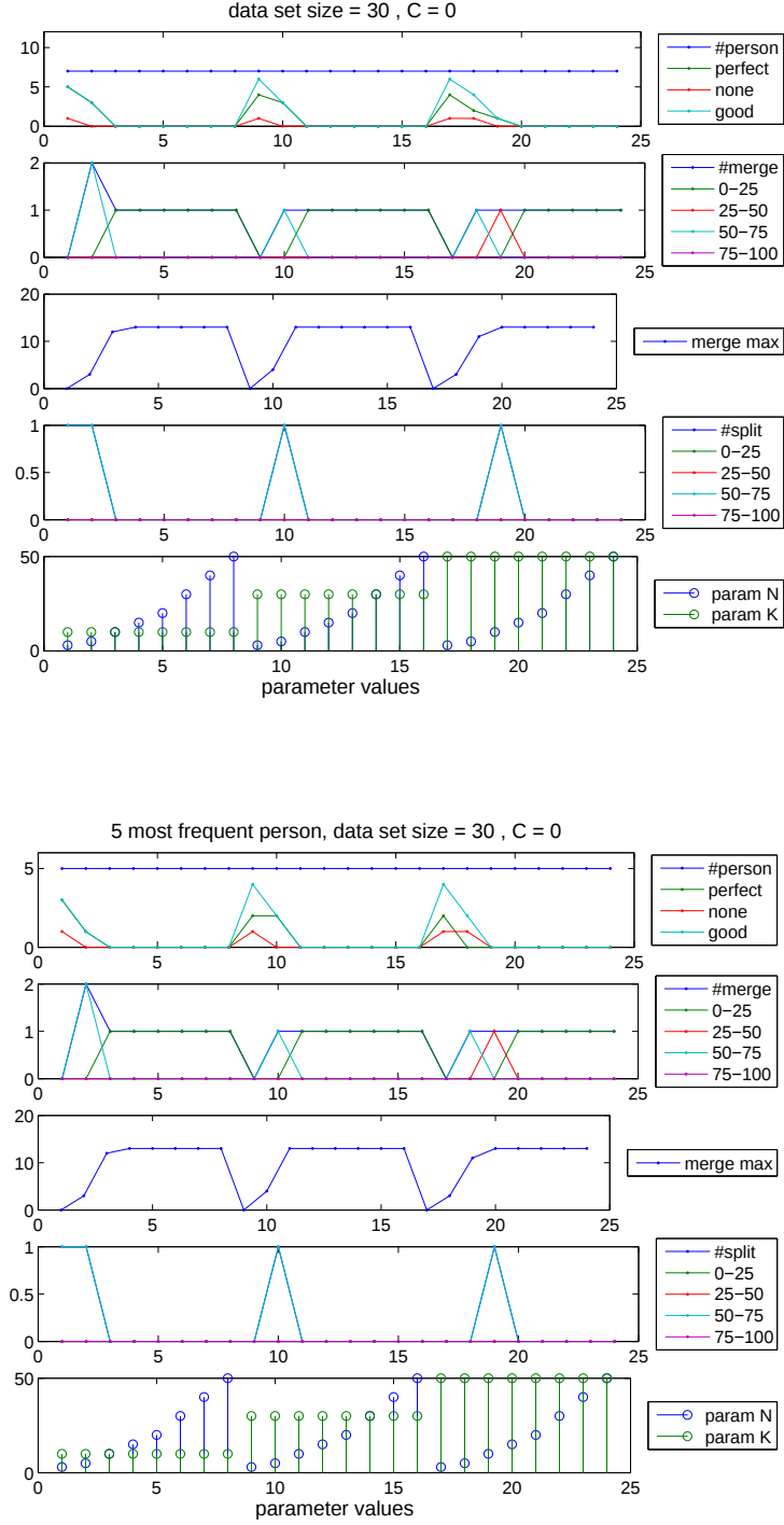
Figure C-1: Results of clustering evaluation of a data set of 30 sequences, C = 0\% . The upper figure shows the results from the entire data set and the lower figure shows a subset of the results from 5 individuals who have the most number of sequences in the data set. The top most subplot illustrates the number of good , perfect , and none resulting clusters. The second subplot shows the number of total merging errors and their distribution for different merge purity values. The third subplot shows the number of merged maximum. The fourth subplot shows the number of splitting errors and their distribution for different split degree values. The rest of the plots in this section follows the same structure.
