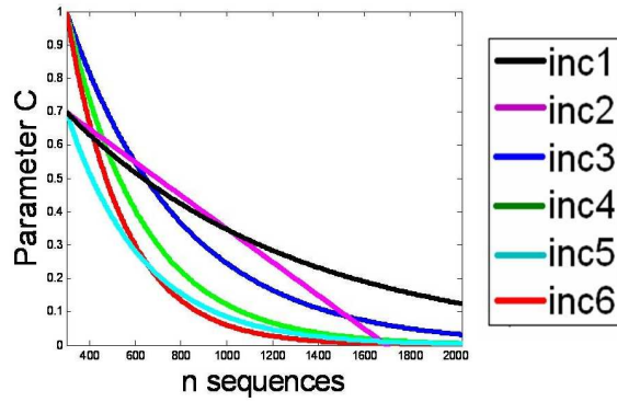
Figure 5-29: The set of correlation functions between the data set size and parameter C values used to evaluate the incremental clustering results.
