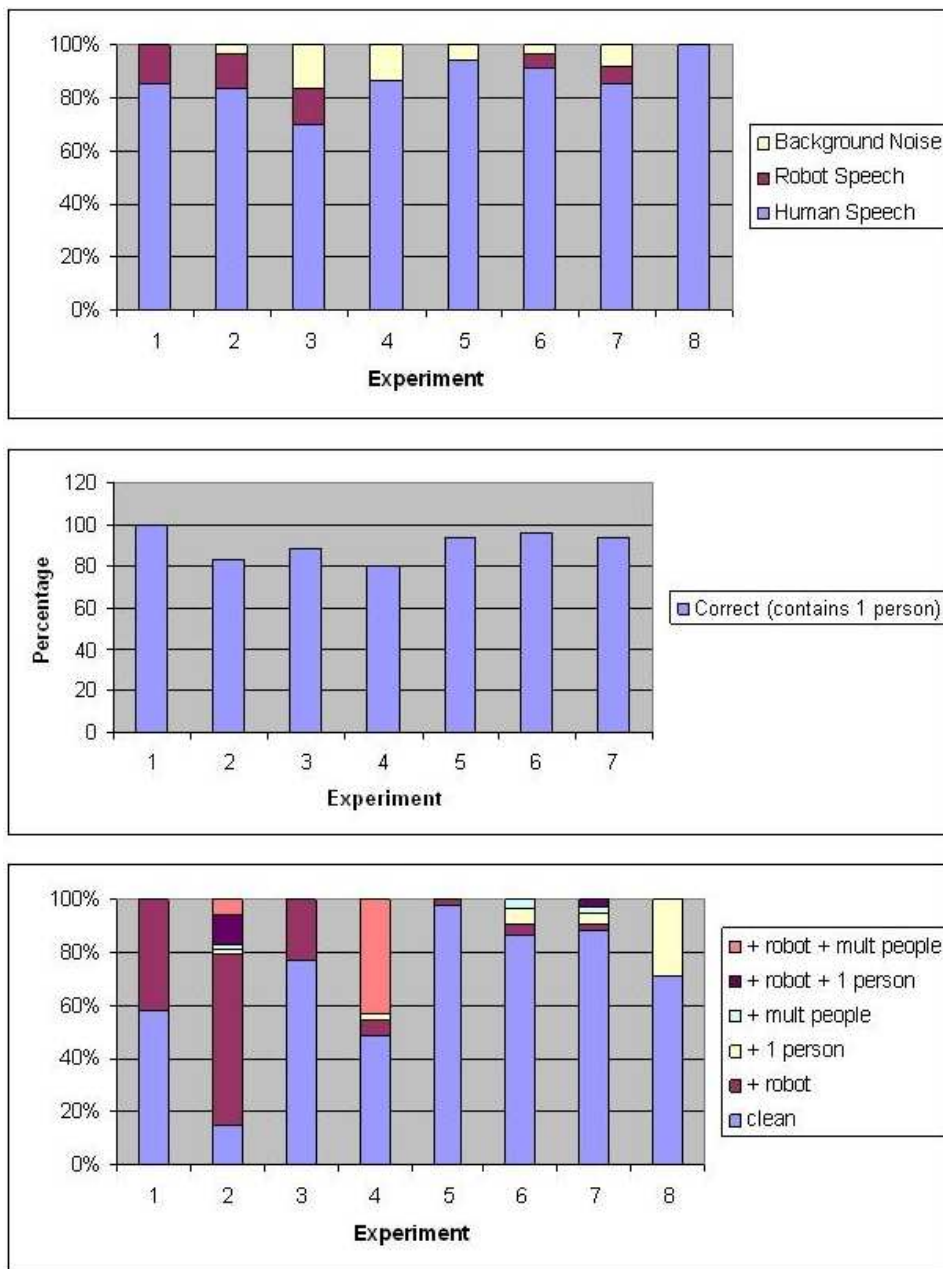
Figure 4-14: Segmentation and Correlation Accuracy of the Paired Face and Voice Data
