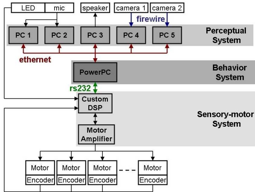
Figure 3-4: The robot's hardware and software control architecture. Rectangular units represent hardware components. The superimposed grey patches represent the software systems implemented on the corresponding hardware. We carefully designed each control layer to be modular and independent. Higher level control layers can be removed at any point without disrupting the robot's operation.
