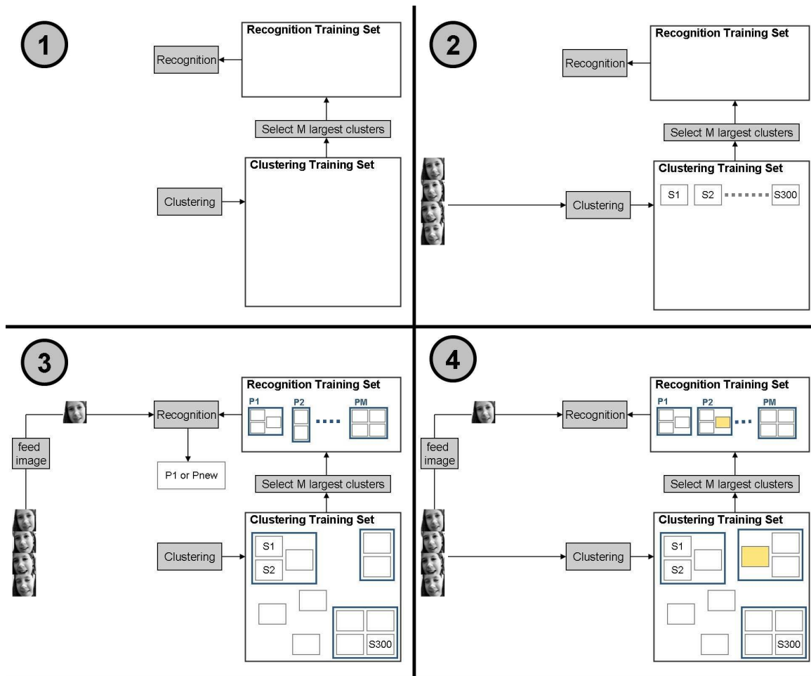
Figure 5-18: The four phases of the unsupervised and incremental face recognition process. During this incremental process, the system builds a labelled training set using self-generated clusters and then uses this training set to recognize each sequence input.
