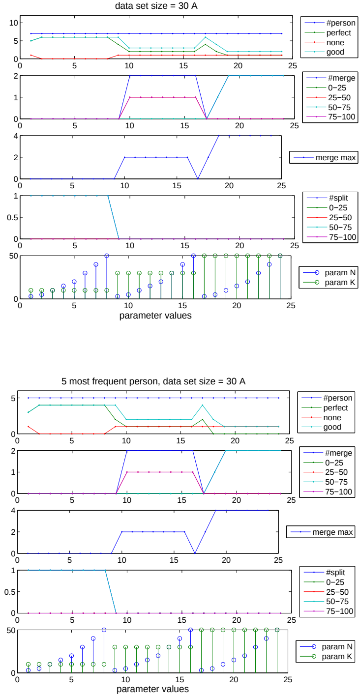
Figure C-2: Results of clustering evaluation of a data set of 30 sequences, C = 70\% . The upper figure shows the results from the entire data set and the lower figure shows a subset of the results from 5 individuals who have the most number of sequences in the data set.
