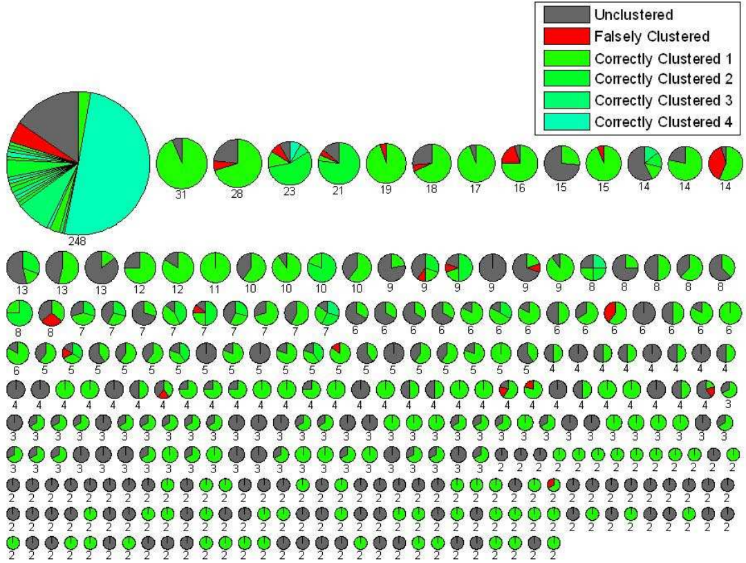
Figure 5-23: Visualization of the self-generated clusters. Each pie chart corresponds to an individual. The size of the pie chart circle corresponds to the number of sequences an individual have in the data set. The different shades of green regions correspond to sequences that were correctly clustered. Multiple green slices are present within a pie chart indicate that there is a splitting error. The red regions correspond to sequences that were falsely clustered, i.e. the merging errors. The gray regions correspond to unclustered sequences.
