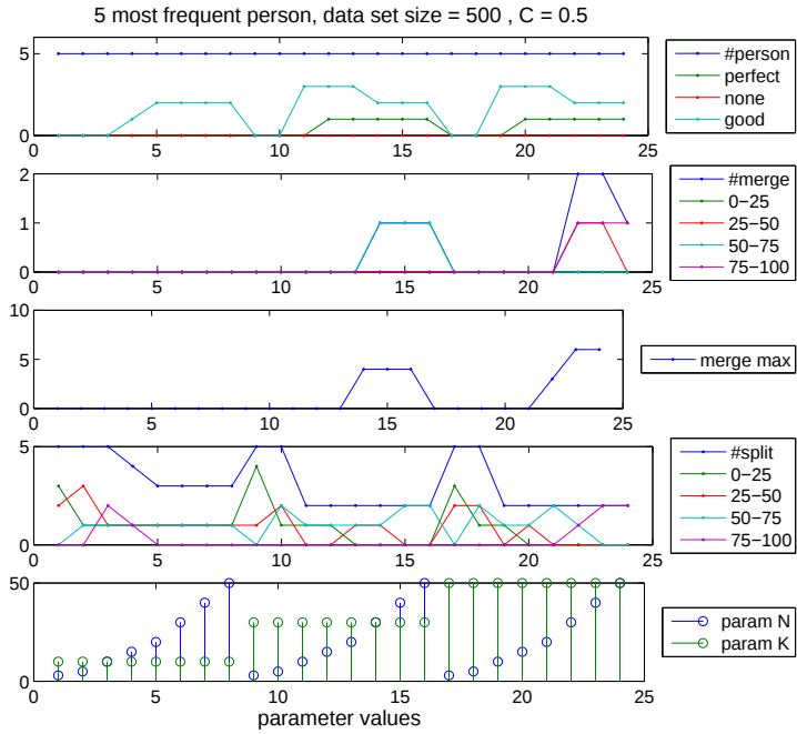
Figure C-17: Results of clustering evaluation of a data set of 500 sequences, C = 50\% . The upper figure shows the results from the entire data set and the lower figure shows a subset of the results from 5 individuals who have the most number of sequences in the data set.
