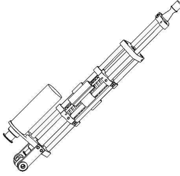
Figure 3-3: The Series Elastic Actuator (SEA) is equipped with a linear spring that is placed in series between the motor and load. A pair of SEAs are used to construct the differential neck joint, allowing easy implementation of force control. The neck axis is the biggest joint responsible for supporting the weight of the head. Thus, the compliancy and ability to maintain position in the absence of power provided by the SEA are particularly useful.
