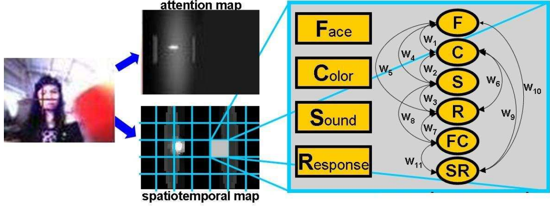
Figure 4-6: A diagram of the robot's spatio-temporal learning map. It consists of a 2D rectangle with 70x52 pixels. Each pixel spatially represents a 4x4 pixels corresponding region in the robot's attentional map. Each map pixel is a storage space, containing four cells, one for each input type (face, color, sound, response), and a hebbian network.
