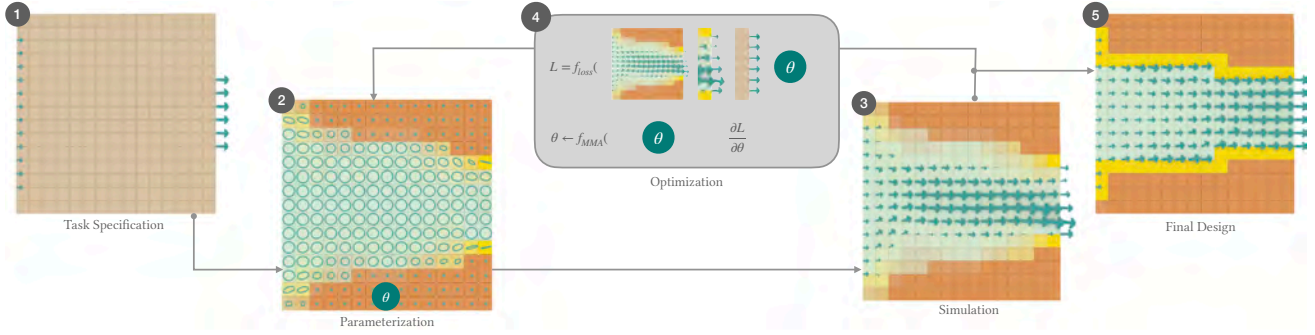
Fig. 2. An overview of our pipeline: (1) Our system takes as input the specification of a fluidic device design task on a regular grid, including the locations and desired profiles of the Stokes flow at the inlet and outlet; (2) The system then represents the fluidic device using anisotropic materials in each voxel, which we further parametrize using its anisotropic direction (the principal axes of the ellipse in the illustration), viscosity (radius of the ellipse), and impedance for fluid (shown as the background color of the voxel); (3) A numerical differentiable simulator receives the design and solves the Stokes flow; (4) The pipeline then compares the simulated flow at the outlet with the target profile given in the specification and computes a loss function characterizing their discrepancy. The loss is then backpropagated through the numerical simulator to compute its gradients with respect to the anisotropic material parameters. The pipeline runs the method of moving asymptotes (MMA, [Svanberg 1987]), a gradient-based optimizer, to improve the design; (5) The pipeline outputs a final design after post-processing the results from a converged optimization process.
