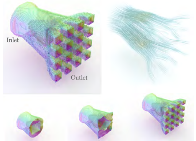
Fig. 5. Our pipeline generates a tree diffuser on a 80 \times 80 \times 80 grid. Top left: The anisotropic boundary of the optimized design is visualized using small colored disks. Bottom: The 3 images in the middle visualize the perpendicular cross-sections of the optimized design at different depths from the inlet. These cross-sections highlight the progressive branching from a single inlet to multiple outlets. Top right: The fluid flow, simulated from the optimized design, is visualized as streamlines.
