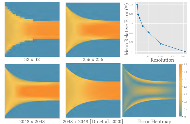
Fig. 7. Evaluation of our solver on a 2D fluid amplifier design. We visualize the norm of the nodal velocity field simulated in square domains of dimension 32, 256 and 2048 (top left, top middle, bottom left). The relative error (to the solution at dimension 2048) monotonically decreases as the resolution increases. We additionally simulate the same design at 2048x2048 using a traditional Stokes flow solver from Du et al. [2020] (bottom middle), and visualize the difference field (bottom right, normalized to inflow value).
