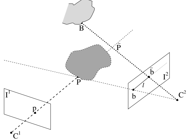
Figure 2.1: Visibility-based segmentation. Observation of \mathbf{B} in C^2 allows us to infer that \mathbf{P} in C^1 is foreground. Point \mathbf{B} visible in I^2 (projecting to C^2 disparity point \bar{\mathbf{b}} ) lies behind point \overline{\mathbf{P}} relative to C^2 , and thus provides evidence for existence of free space behind \mathbf{P} (projecting to \mathbf{b} ) by demonstrating that \overline{\mathbf{P}} is transparent. Line l contains the overshilhouette for the part of an object lying along ray [C^1, \mathbf{P})
