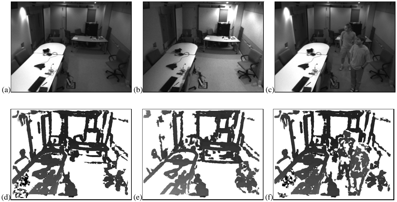
Figure 4.1: Intensity and disparity pairs obtained from camera C^1 . (a, d) – empty room. (b, e) – empty room under different lighting conditions. (c, f) room with two people. The pixels with invalid disparity are shown in white.
