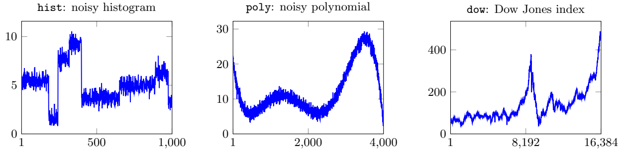
Figure 1: Data sets for the offline histogram approximation experiments. (left) hist is a histogram consisting of 10 pieces contaminated with Gaussian noise ( n = 1000 ). (middle) poly is a degree 5 polynomial, also contaminated with Gaussian noise ( n = 4000 ). (right) dow is a time series of Dow-Jones Industrial Average (DJIA) daily closing values ( n = 16384 ).
