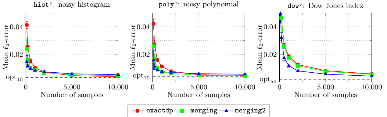
Figure 2: Results of the histogram learning experiments for three different data sets (see Figure 1). Every data point is the mean error over 20 trials and the error bars indicate one standard deviation. The \text{opt}_k values are the approximation error of the best k -histogram fit to the underlying distribution.
