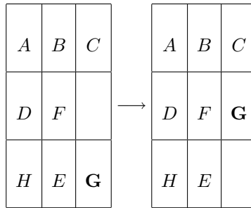
Figure 3.10: An example of a column move in which the G -tile is moved into the adjacent hole above. In this case, G changes order with E and H .
