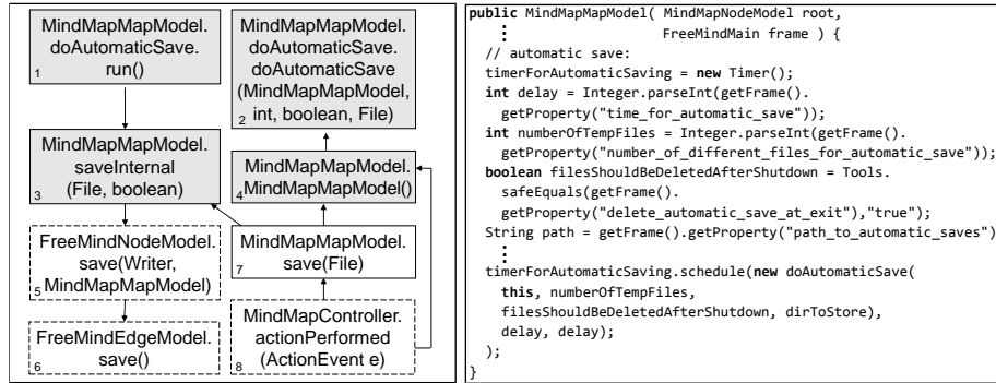
Fig. 1 The automatic save file call graph snippet.
