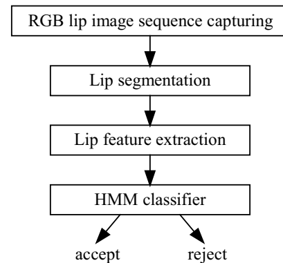
Fig.1 Flowchart of the speaker authentication system
