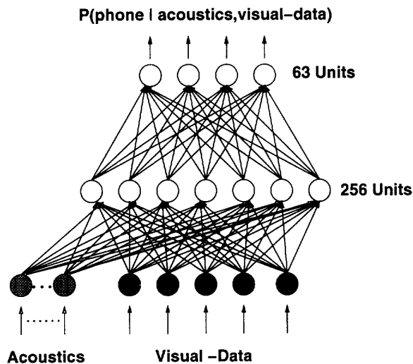
Figure 3: Connectionist architecture.
