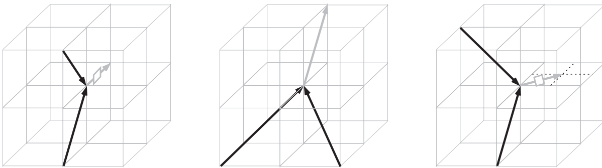
Figure 4: 3D Soft Sphere Models. (a) Collisions using cube edges and cube-face diagonals. Each edge particle carries one bit of information about which of two planes the diagonal particles that created it were in. (b) Collisions using face and body diagonals. Two body-diagonal particles collide only if they are both coplanar with a face-diagonal. The resulting face-diagonal particle doesn't carry any extra planar information, since there is a unique pair of body-diagonal particles that could have produced it. (c) Collisions using only face diagonals, with two speeds. If particles are confined to a single plane, this is equivalent to the triangular lattice model of Figure 3b. Again the slower particle must carry an extra bit of collision-plane information.
