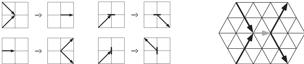
Figure 3: (a) A simple lattice gas rule captures the dynamics of the soft sphere collision. Two particles colliding at right angles turn into a single new particle of twice the mass for one step, which then turns back into two particles. A mirror deflects a particle through 90^\circ . In all other cases, particles go straight. (b) A soft sphere collision on a triangular lattice.
