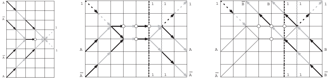
Figure 14: A way to reflect signals back, without refining the lattice or adding extra particles. (a) If we have two dual rail signal-pairs (one the complement of the other), then they can be bounced straight backward along the same paths they came in on by bringing all the signals to one point at which two mirror signals impinge. In either case ( A=0 and A=1 ), the constant 1's that reflect these signals are also reversed along their paths. (b) The thick vertical dotted line-segments indicate constants of one that are moving in both directions at the indicated locations. This is otherwise a normal reflection of a signal—the extra vertical streams don't interfere with the operation of the “mirror.” (c) If a backward propagating signal comes in from the right ( B and \bar{B} ), then it is not reflected by this forward mirror—such a mirror separates the backward moving stream from the forward stream.
