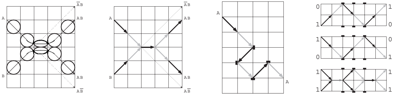
Figure 2: A soft sphere model of computation. (a) A BBM-like collision using very compressible balls. The springiness of the balls is chosen so that after the collision, the balls are again at integer sites at integer times. The logic is just like the BBM, but the paths are deflected inwards, rather than outwards. (b) Arrows show the velocities of balls at integer times. During the collision, we consider the pair to be a single mass, and draw a single arrow. (c) We can route and delay signals using mirrors. (d) We can make signals cross.
