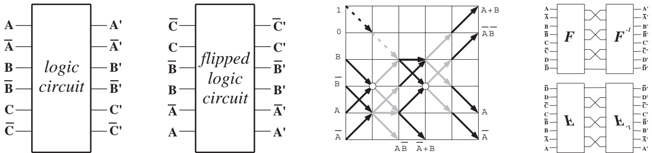
Figure 15: DeMorgan inversion. (a) A logic circuit with dual-rail inputs. In each input pair, the complemented signal lies below the uncomplemented one. (b) If this circuit is flipped vertically, the operation of the circuit is unchanged, but it operates upon inputs that are complemented (according to our conventions) and produces outputs that are also complemented. (c) The switch gate of Figure 8a, flipped vertically. Inputs and outputs have been relabeled to call the top signal in each dual-rail pair “uncomplemented.” (d) The BBMCA logic circuit of Figure 10b has been mirrored vertically to produce a vertically symmetric circuit which has complementary pairs of dual-rail pairs.
