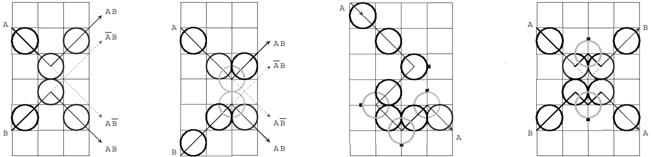
Figure 1: The Billiard Ball Model. Balls are always found at integer coordinates at integer times. (a) A collision that does logic. Two balls are initially moving towards each other to the right. Successive columns catch the balls at successive integer times. The dotted lines indicate paths the balls would have taken if only one or the other had come in (i.e., no collision). (b) Balls can collide at half-integer times (gray). (c) Billiard balls are routed and delayed by carefully placed mirrors as needed to connect logic-gate collisions together. Collisions with mirrors can occur at either integer or half-integer times. (d) Using mirrors, we can make two signal paths cross as if the signals pass right through each other.
