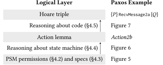
Figure 2: A layering overview of the permissioned state machine approach. Each layer above an arrow is proved using the layer below it.
