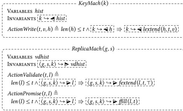
Figure 25: Partial PSM specifications capturing read correctness. The function extend ( h, t, v ) first fills value history h through index t − 1 using its last value (or the “tombstone” record if the key has not been written before), and then appends v . The function extend ( l, t, b ) fills list l through index t − 1 using \perp , and then appends b . The function fill ( l, t ) performs only the filling step of extend .
