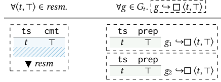
(b) An example state satisfying InvCommit , with G_t = \{g_1, g_2\} .
