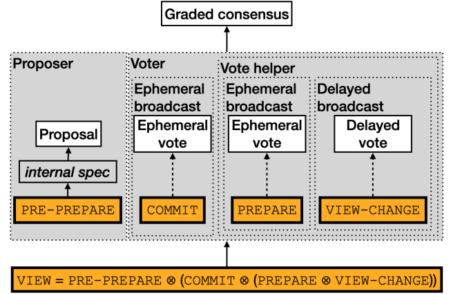
Figure 1: Modules in Shipwright as they are used to verify a single view of PBFT. \otimes is Shipwright's composition operator. (Not shown is how an infinite sequence of views compose into a single run of PBFT.) There is one module for each message type in PBFT, and the implementation of the entire view is constructed with synchronous dispatch into the implementations of each module. Only the internal structure of the top-level module and the PRE-PREPARE-to-“proposal” submodule are shown; all others are encapsulated.
