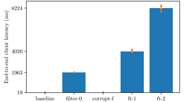
Figure 13: End-to-end latency of a client request under a variety of scenarios representing different attacks, given f = 2 . In the first scenario, an attacker intermittently prevents the delivery of COMMIT messages in view 0, but the system recovers shortly afterwards. In the second, the attacker controls two nodes. In the last two scenarios, both the network attack and node corruption take place (for one and two nodes, respectively).
