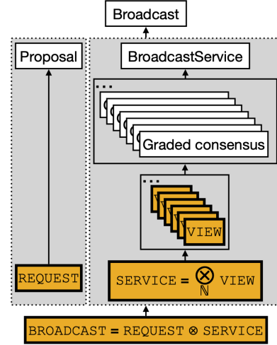
Figure 10: A diagram of the refinement proof's compositional structure; Figure 1 shows the detailed structure of the refinement between a single view implementation and a single graded consensus spec.
