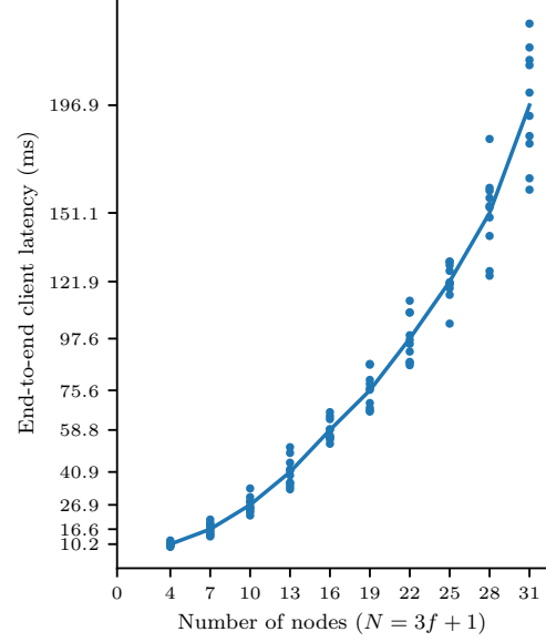
Figure 12: End-to-end latency of a client request in a system with N = 3f + 1 nodes, varying values of f from 1 to 10 for 10 iterations each. The scatter plot represents the raw data while the line plot represents averages. The labels on the y-axis correspond to the averages.
