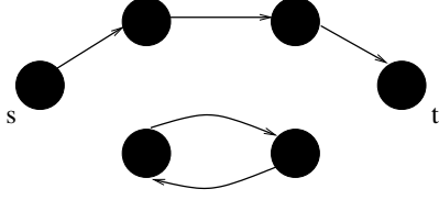
Figure 1: A subgraph that contains a cycle, while satisfying constraints 2 through 5.
