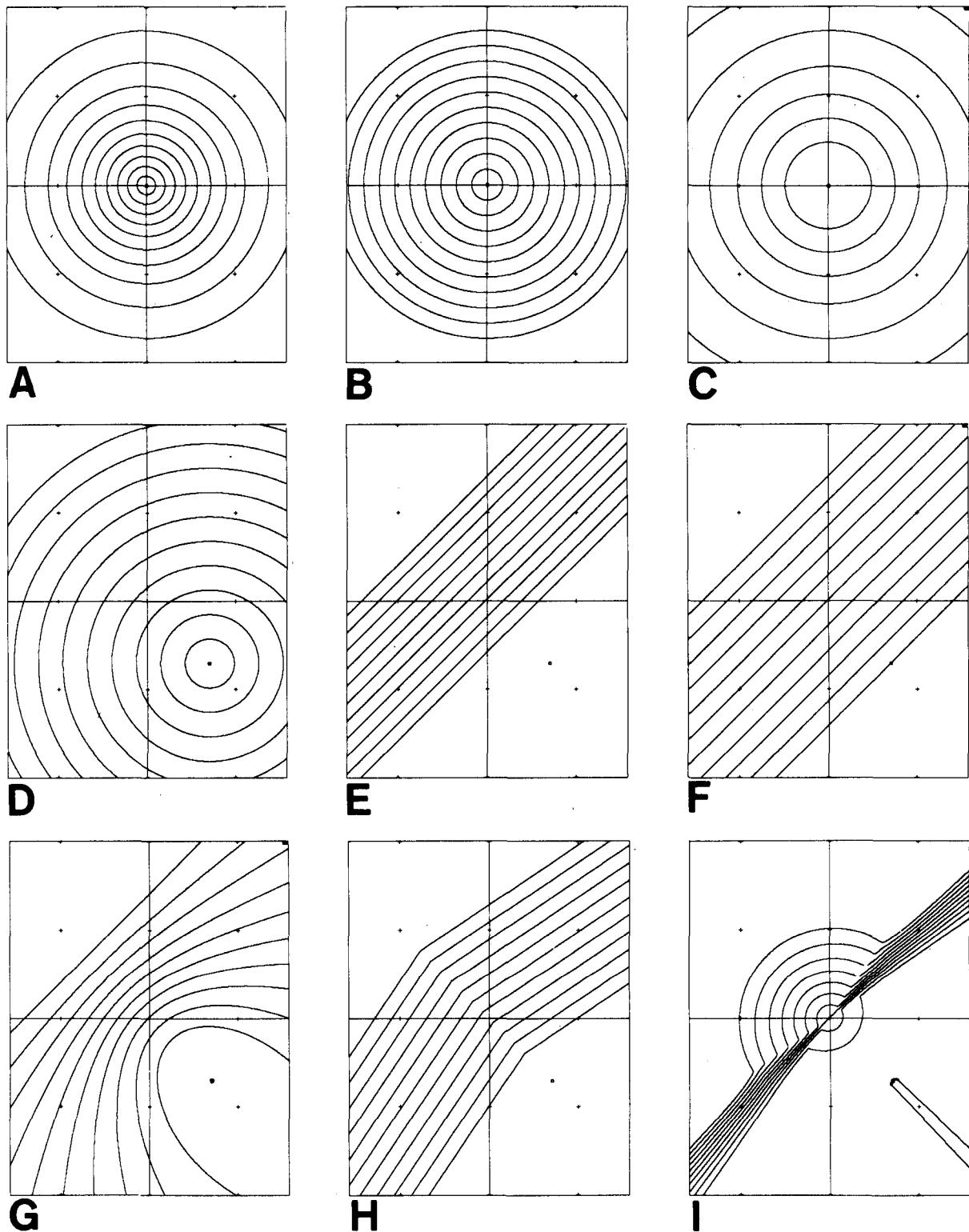
Fig. 19. Reflectance maps in the order in which they were introduced. The letter codes on subfigures match the letters found after the headings of corresponding sections of this paper. Small crosses mark points in gradient space where slope-components are integer multiples of 1. Where appropriate, a small square marks the gradient of a surface element that is perpendicular to the rays from the assumed light-source.
