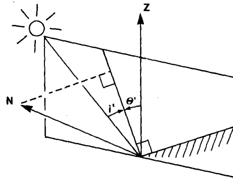
Fig. 15. Projection of the surface normal on a vertical plane containing the assumed light-source. The projected normal is perpendicular to the line in which the plane cuts the terrain surface.
