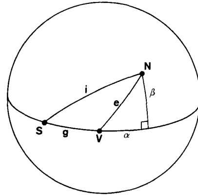
Fig. 25. Luminance longitude \alpha and luminance latitude \beta of a surface element are defined as the longitude and latitude of a patch on a sphere with the same orientation. Longitude and latitude are measured relative to the luminance equator through the light source S and the viewer V .
