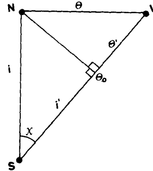
Fig. 16. Spherical triangles used to calculate the projected incident angle i' and the projected surface inclination \theta' . The direction towards the viewer is V , the direction to the source is S , while the surface normal is N .
