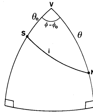
Fig. 13. Spherical triangle used in calculating the incident angle i from the azimuth and elevation of the light-source and the azimuth and elevation of the surface normal. The direction towards the viewer is V , the direction to the source is S , while the surface normal is N .
