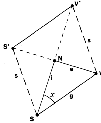
Fig. 17. Spherical triangles used to calculate the first off-specular angle s . It is the angle between S , the center of the source, and S' , the direction from which light is specularly reflected towards the viewer. Equivalently, it is the angle between V , the direction of the viewer, and V' , the direction in which light from the center of the source is specularly reflected.
