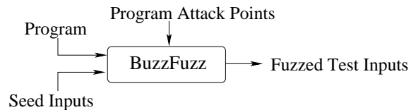
Figure 1. BuzzFuzz Diagram. The inputs to BuzzFuzz are: source of a C program, seed inputs, and a list of program attack points. The output of BuzzFuzz is a set of fuzzed test inputs
