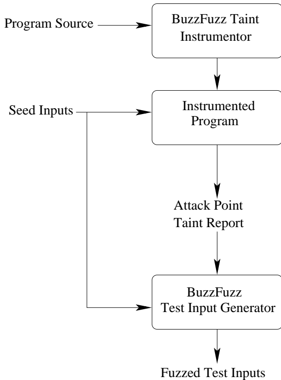
Figure 3. Internals of BuzzFuzz
