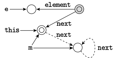
Figure 4: Multiset Example
