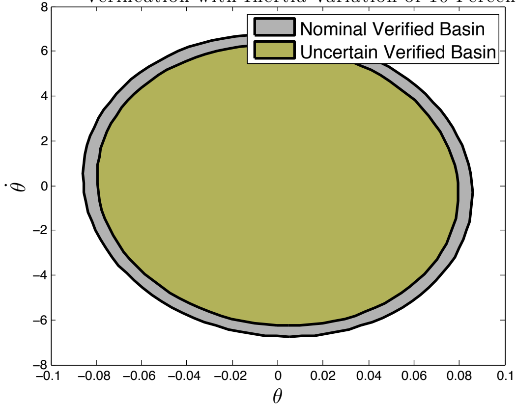
Verification with Inertia Variation of 10 Percent
