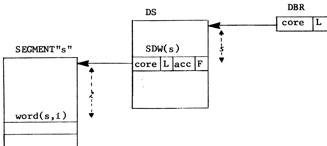
Figure 1. Hardware Segmentation in the 645
