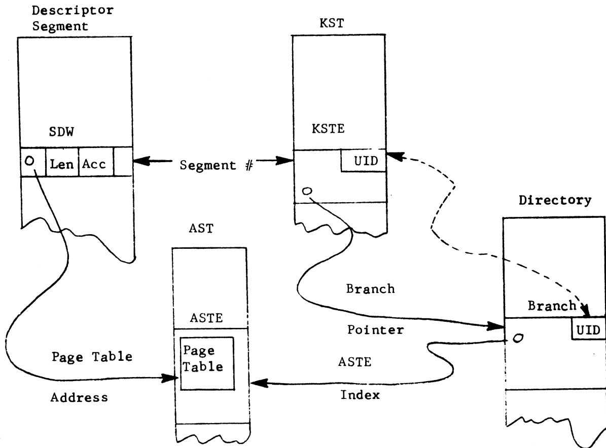
Figure 2. Principal Data Structures Used by the Segment Fault Handler
