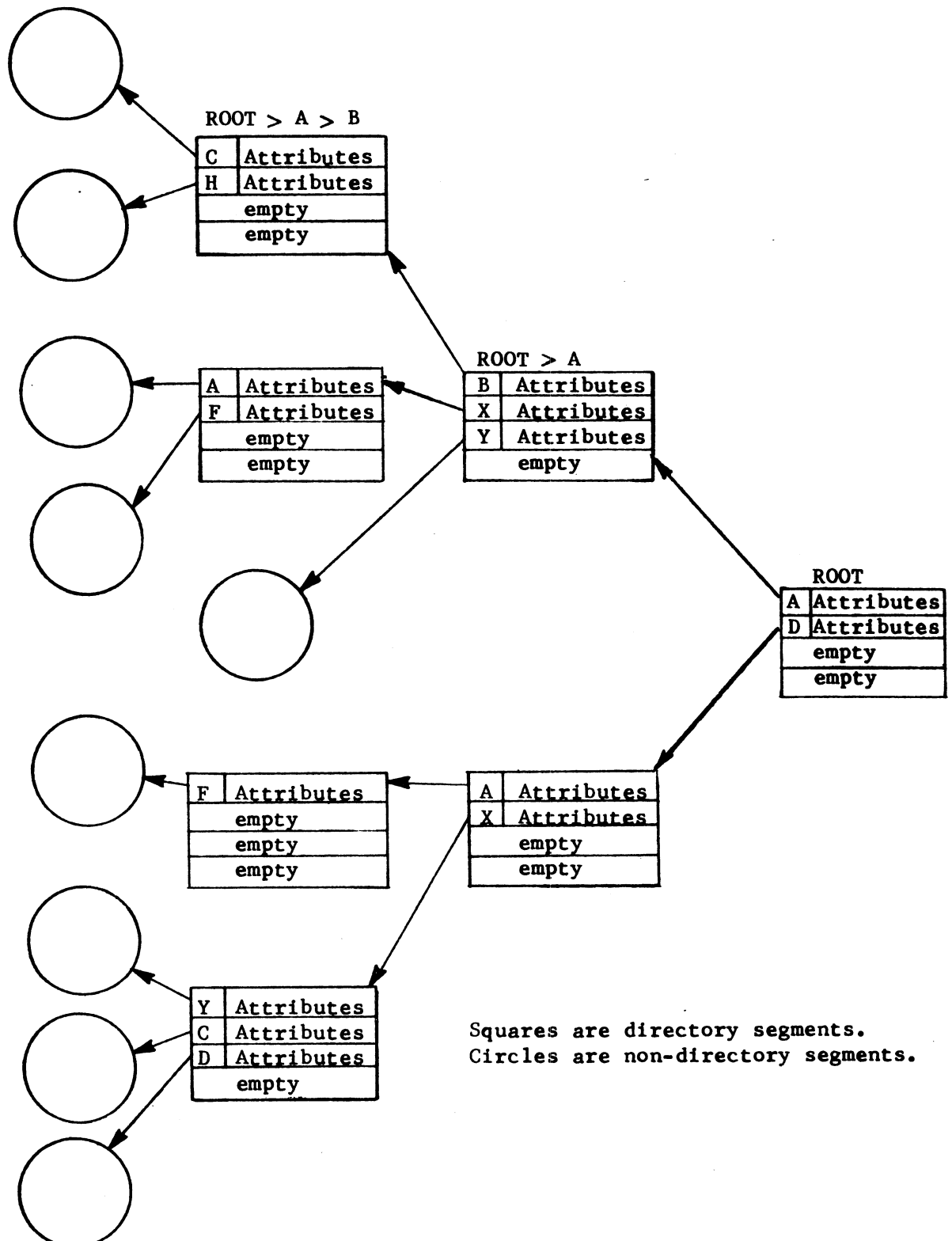
Figure 4. Directory Hierarchy
