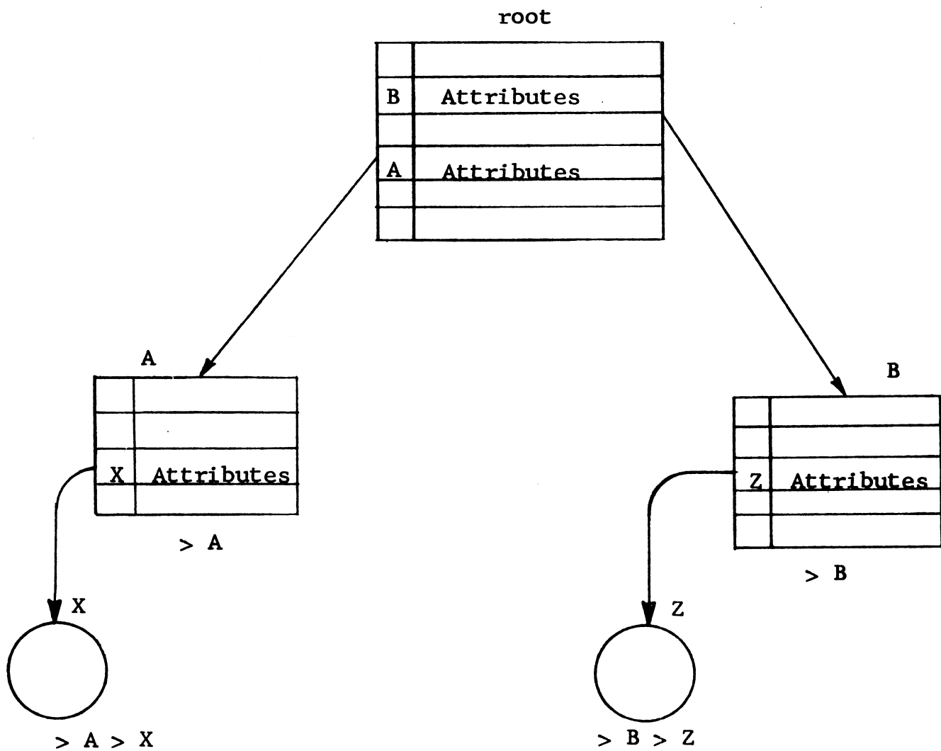
Figure 2. Directories and Attributes
