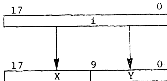
Figure 2. Hardware Interpretation of the Word Number
