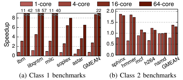
Fig. 15: Performance of T4 on systems with simple in-order cores, normalized to serial code running on the same system.
