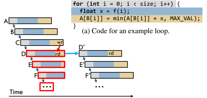
(a) Code for an example loop.
