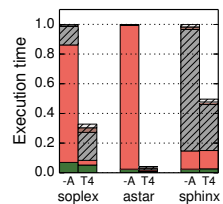
Fig. 13: 64-core execution time without (-A) and with (T4) task-splitting annotations.
