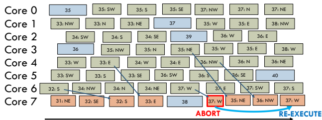
Fig. 9: Execution timeline of astar. Task colors match Listing 1. Numbers denote loop iterations. Arrows indicate spawns of neighbor-append tasks.
