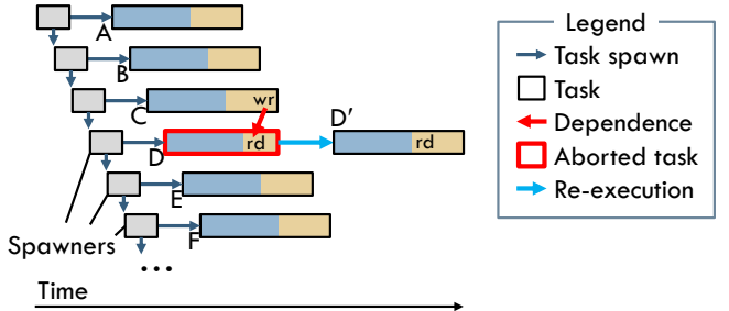
(b) In a TLS task chain, aborting D also aborts later tasks E, F,...
