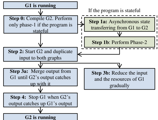
Figure 9. Flowchart of adaptive seamless reconfiguration from old graph instance G1 to new graph instance G2.
