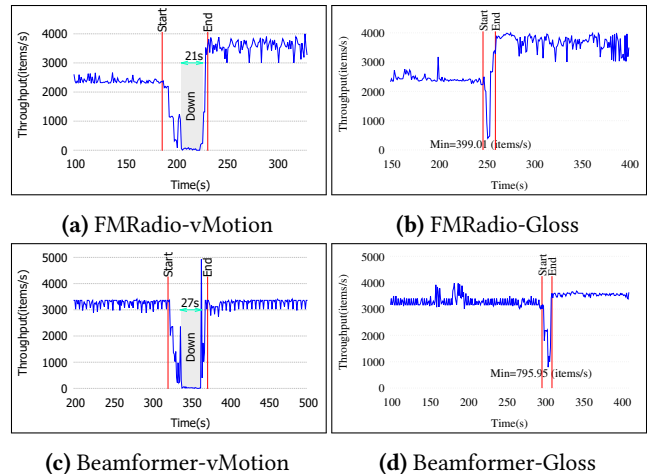
Figure 11. Downtime comparison of vMotion migration and Gloss adaptive seamless reconfiguration for FMRadio (a stateless program) and Beamformer (a stateful program).
