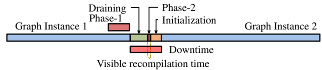
Figure 5. Time breakdown of the two-phase recompilation strategy. The phase-1 compilation happens while the graph instance-1 is running. Only the phase-2 becomes visible and contributes to the downtime.
