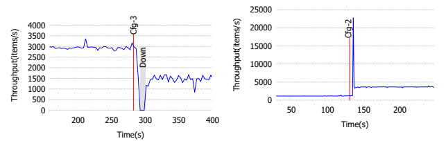
(a) Downtime when transitioning from high to low throughput. (b) Output spikes when transitioning from low to high throughput.
