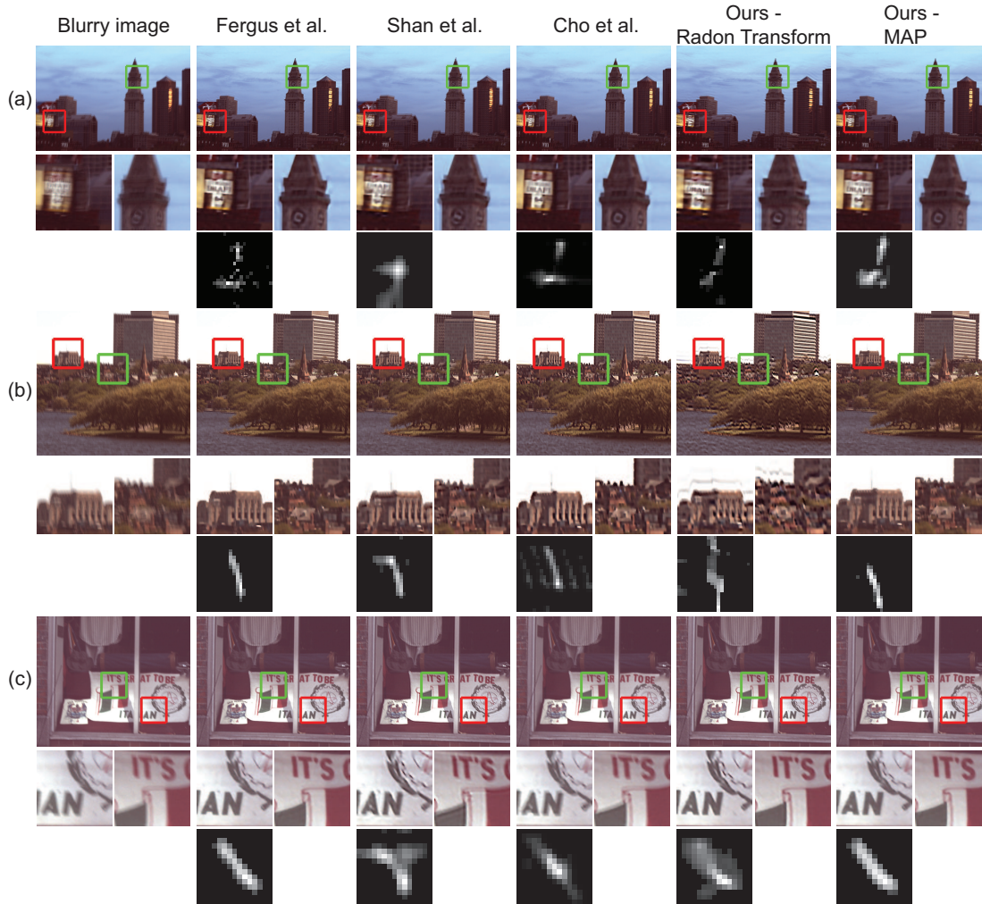
Figure 2.11: By integrating kernel projection constraints to a MAP kernel estimation method, we can improve the kernel estimation performance. We name this algorithm RadonMap . (a-b) show that even when there are not enough edges in different orientations (as shown in Fig. 2.9), the RadonMap algorithm can reliably reconstruct the kernel.
