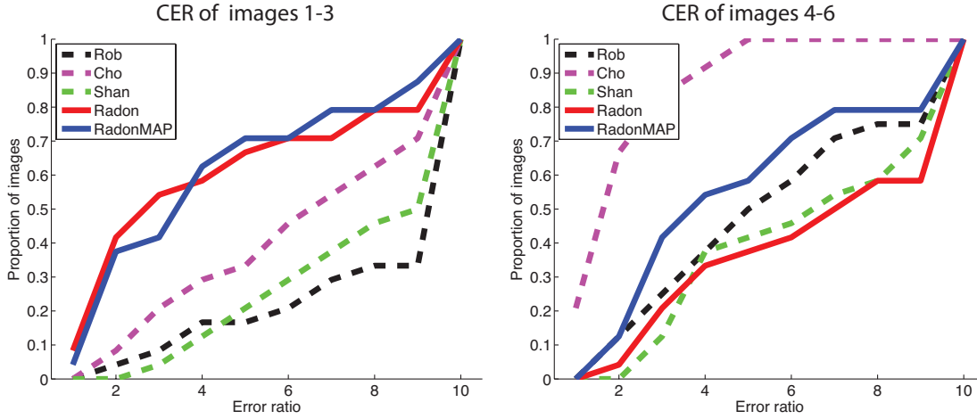
Figure 2.15: In this figure, we plot the cumulative error ratio for images 1–3 and images 4–6 separately. The inverse Radon transform of kernel projections (named Radon) and the MAP estimation with kernel projection constraints (named RadonMAP) both perform well when images contain many edges in different orientations as in images 1–3, but their performance drops drastically when images do not contain enough edges as in images 4–6.
