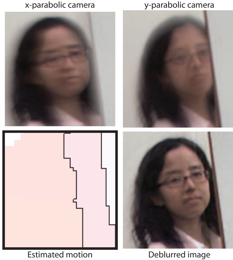
Figure 5.15: Our image reconstruction algorithm handles occlusion boundaries in a manner similar to motion boundaries. In the occluded region, an image deblurred using only one of the two input images is used.
