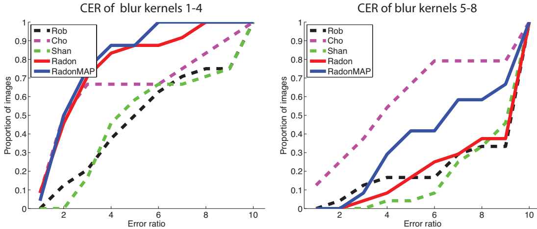
Figure 2.16: The performance of the inverse Radon transform of kernel projections (named Radon) and the MAP estimation with kernel projection constraints (named RadonMAP) depend on the size of the blur. In this figure, we plot the cumulative error ratio for kernels 1–4 and kernels 5–8 in Fig. 2.13 separately. We observe that both Radon and RadonMAP are state-of-the-art when blur kernels are small, but their performance drops drastically when blur kernels are large.
