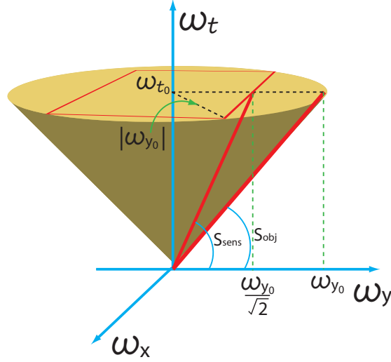
Figure 5.6: The joint spectrum of orthogonal parabolic motions subsumes the wedge of revolution if S_{sens} \geq \sqrt{2}S_{obj} .
