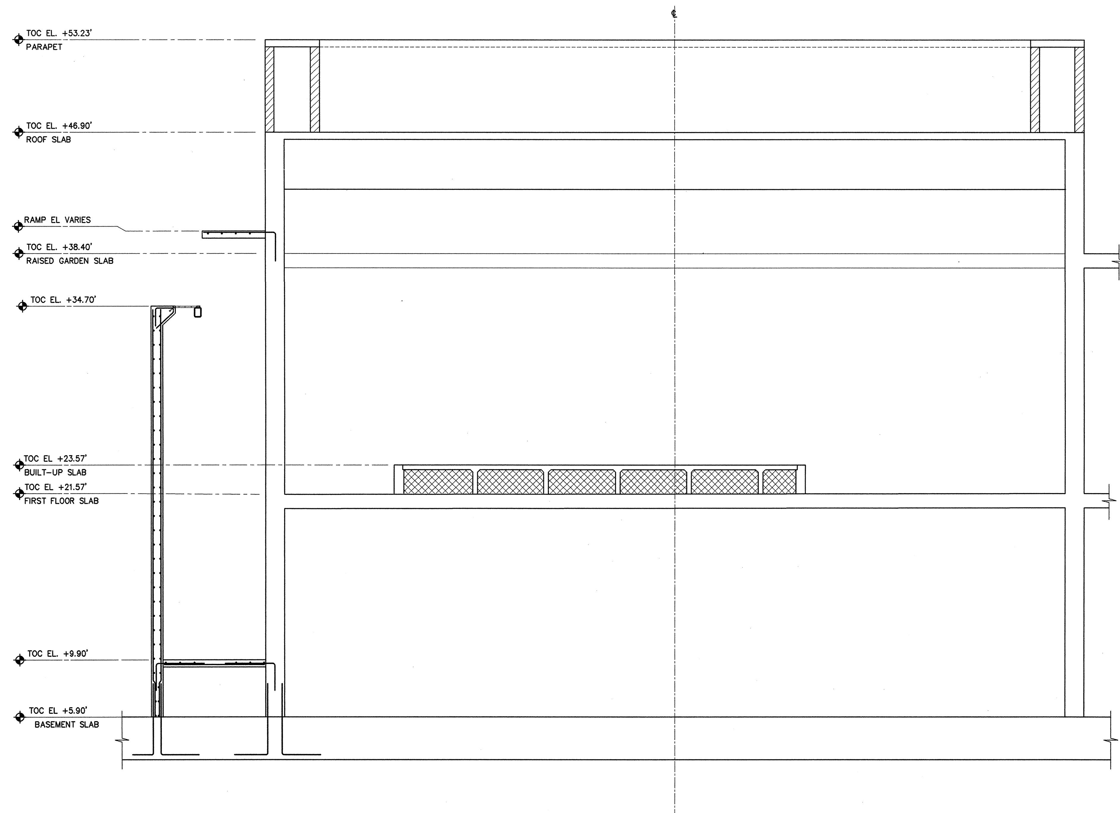
4 SECTION • NORTH WALL 1/4"=1'-0"
