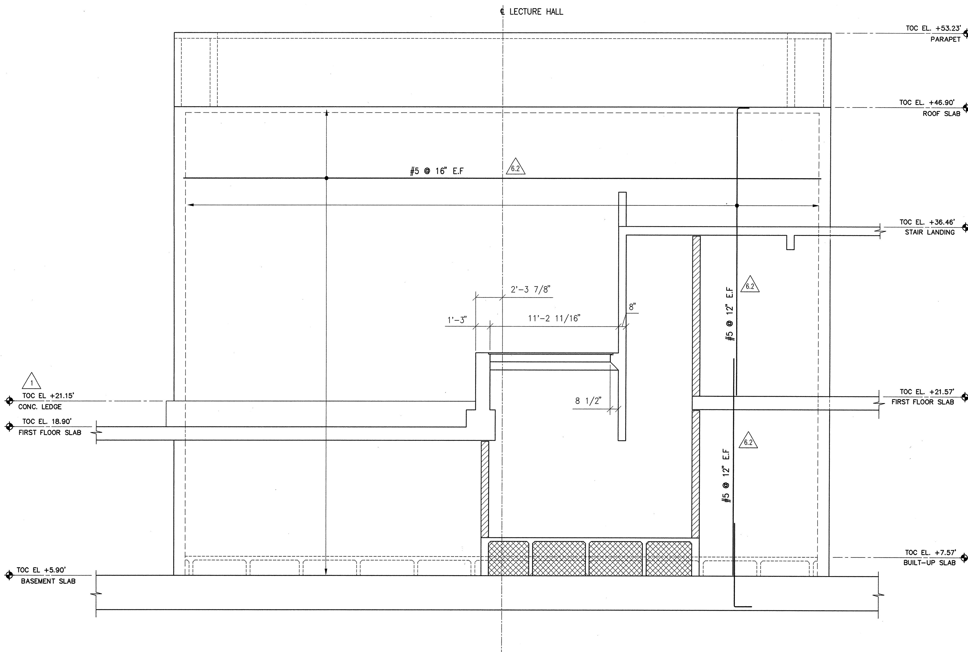
2 SECTION • SOUTH WALL 1/4"=1'-0"
