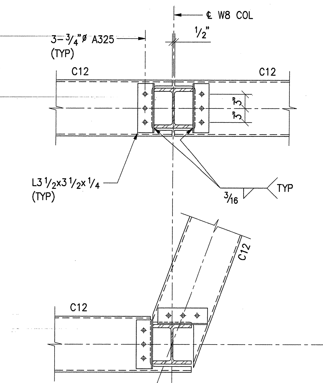
2 PLAN-SECTION 1"=1'-0"
