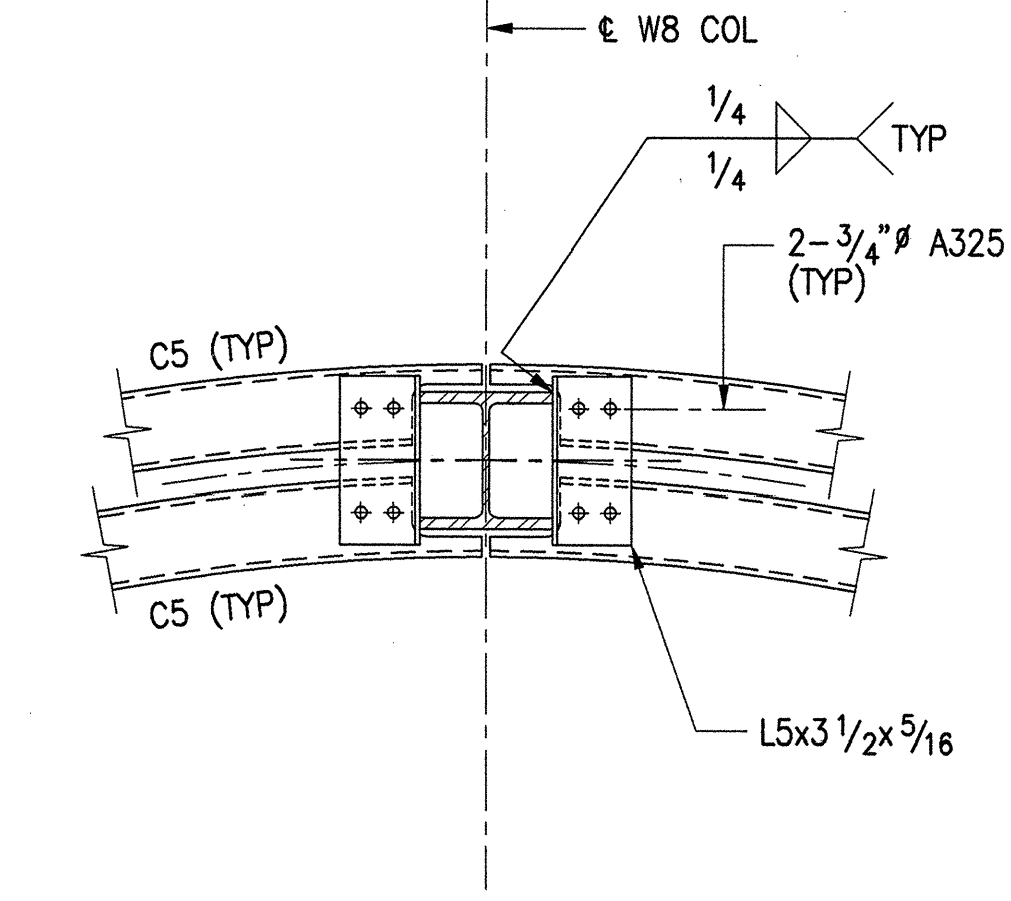
4 PLAN-SECTION 1"=1'-0"
