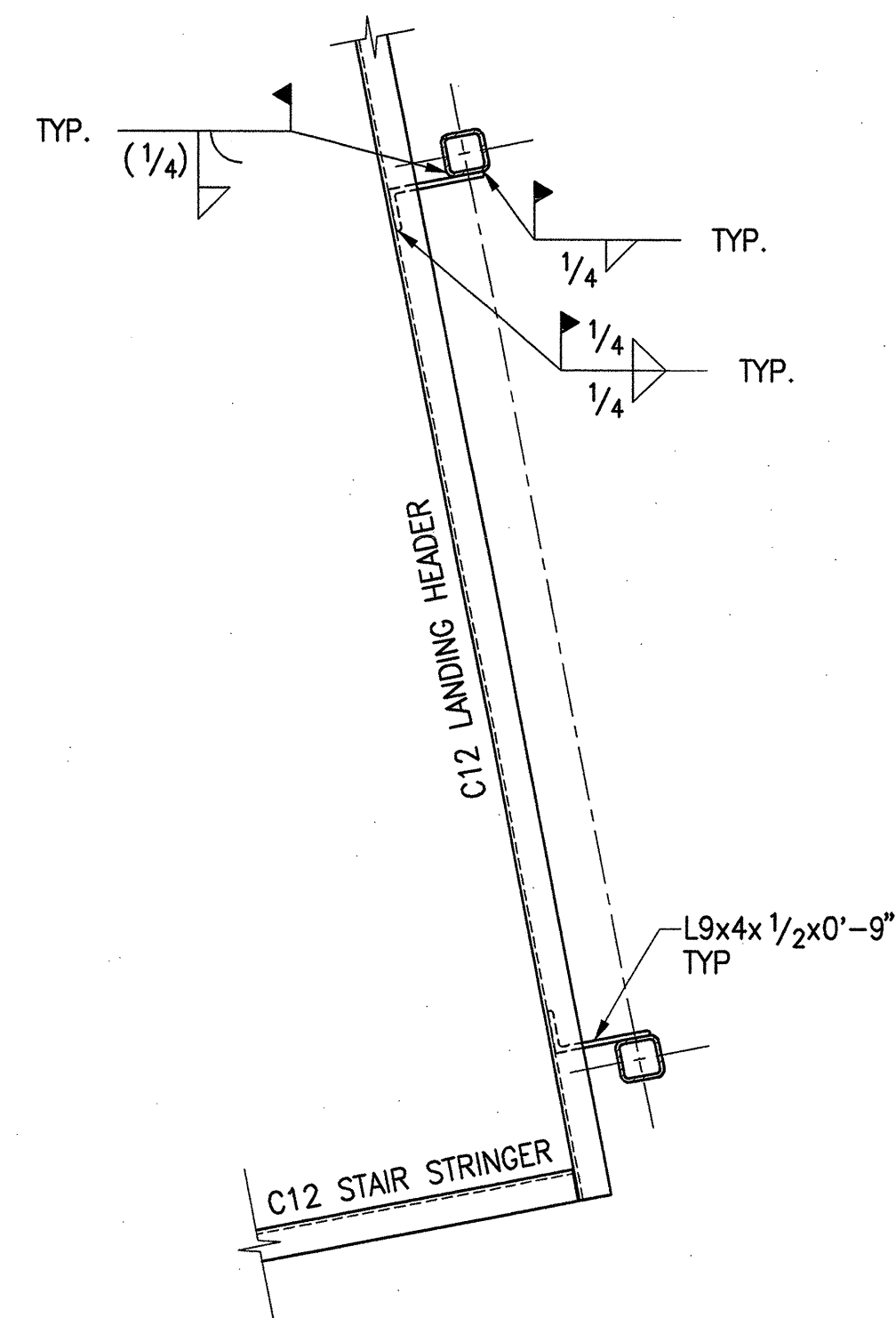
2A STAIR 2 LANDING SUPPORT 3/4"=1'-0"
