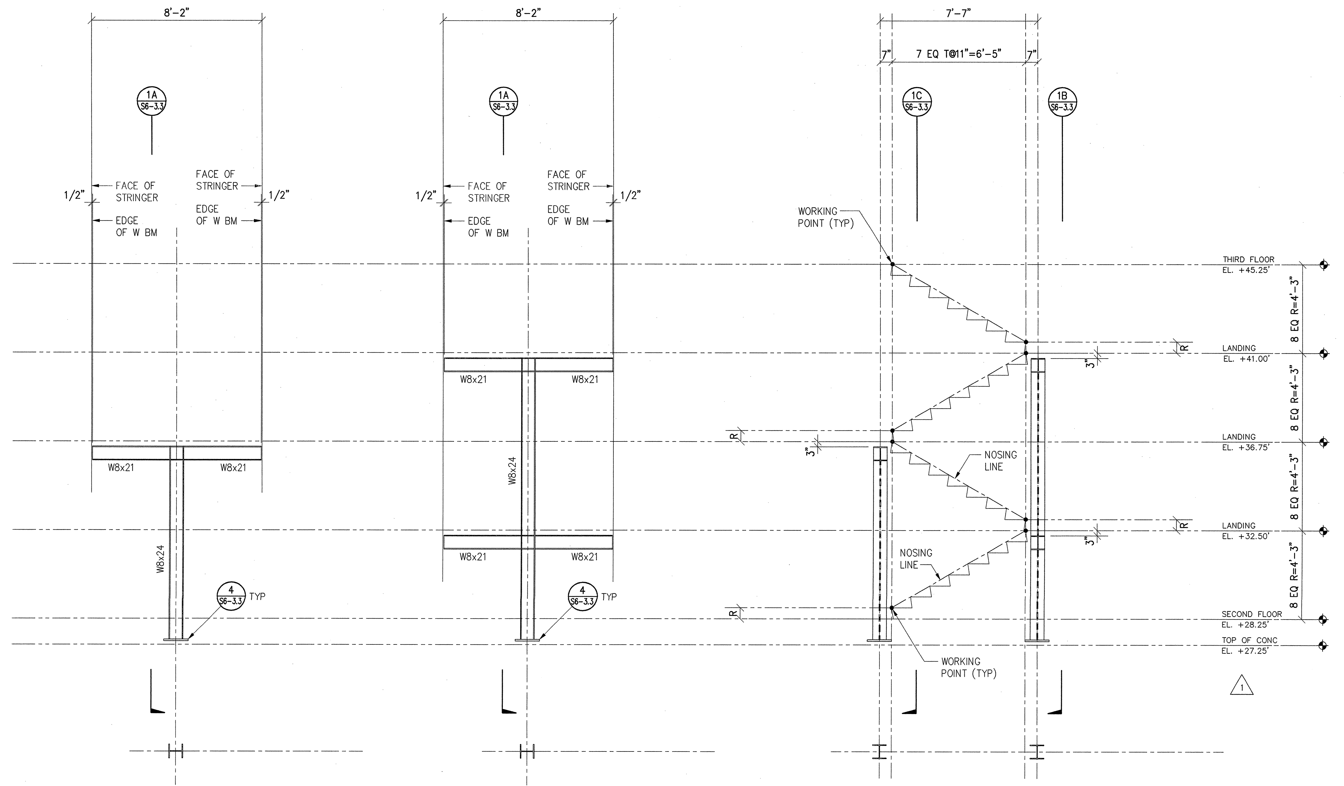
1C SECTION AT STAIRS 13 AND 14 3/8"=1'-0"
