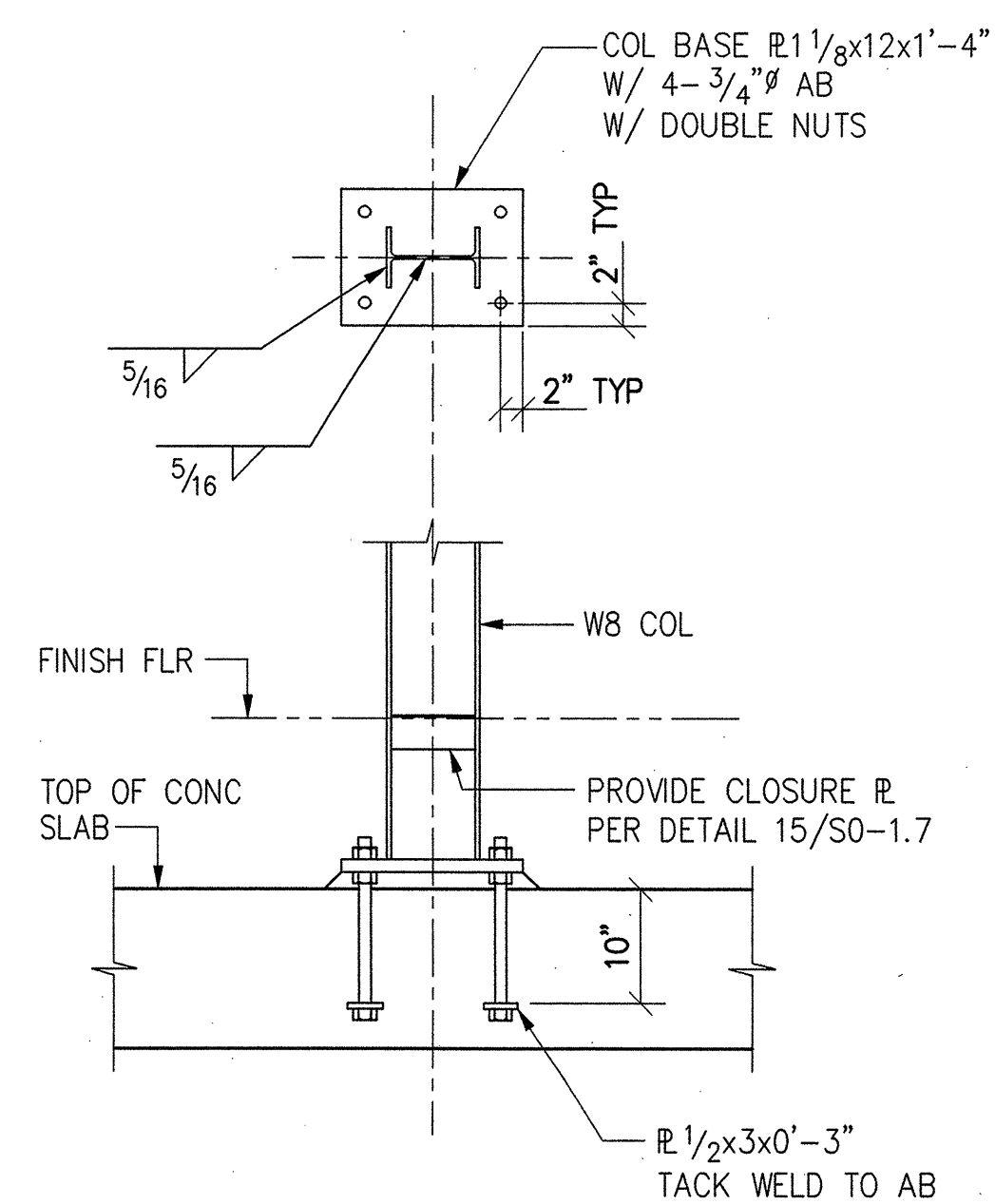
4 DETAIL 3/4"=1'-0"
