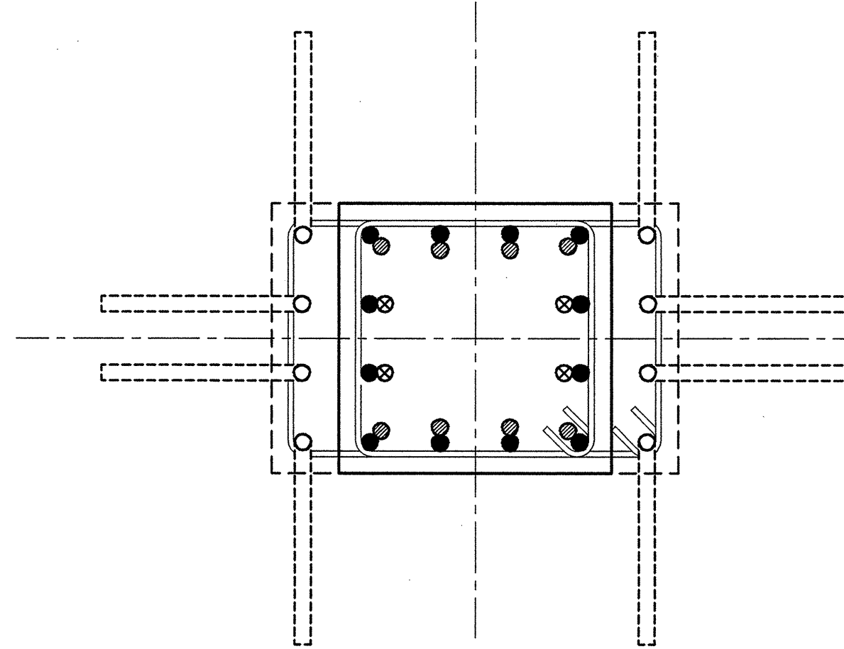
24"x36" TO 24"x24"
