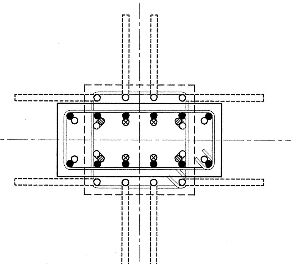
24"x24" TO 16"x36"
