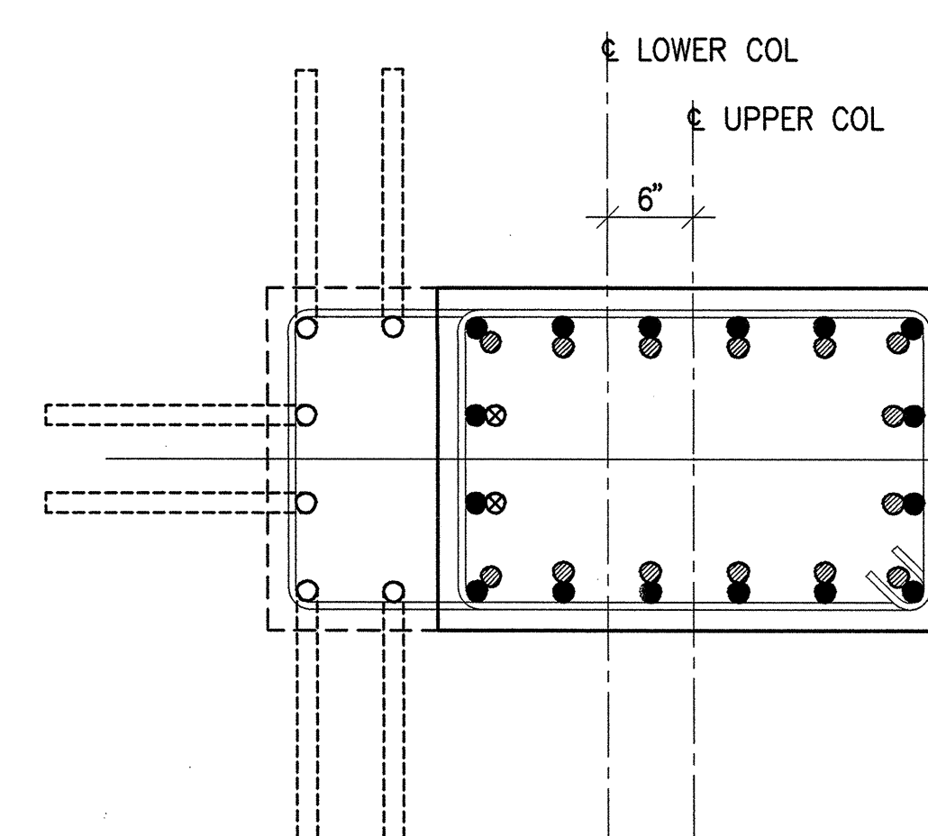
24"x48" TO 24"x36" W/ 6" OFFSET
