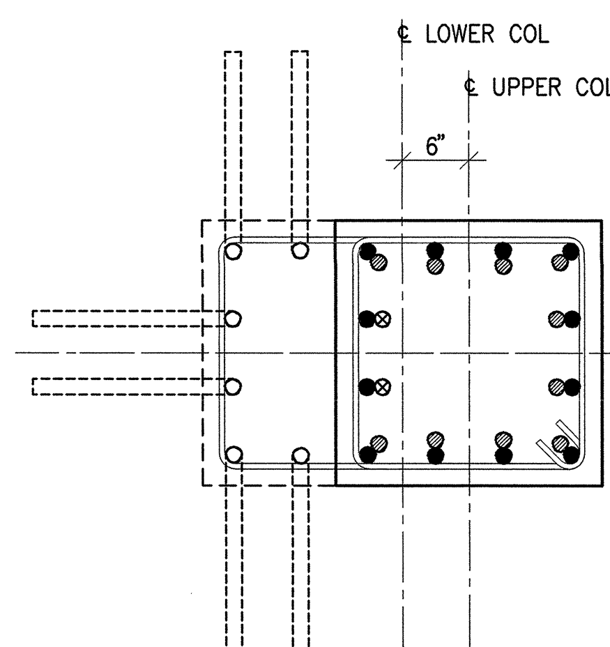
24"x36" TO 24"x24" W/ 6" OFFSET
