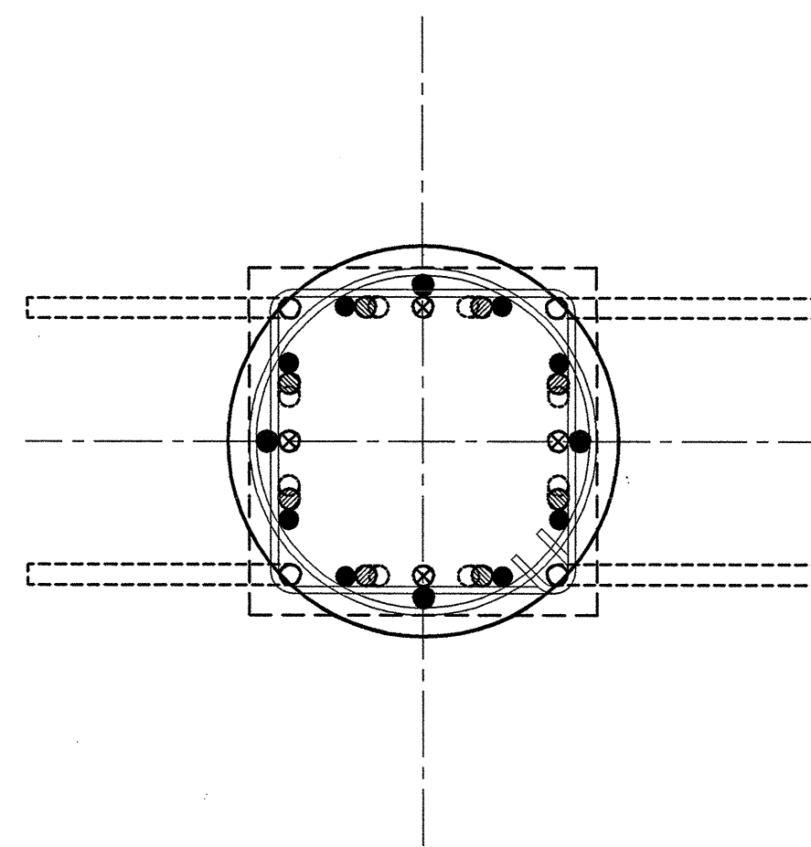
24"x24" TO 27"Ø
