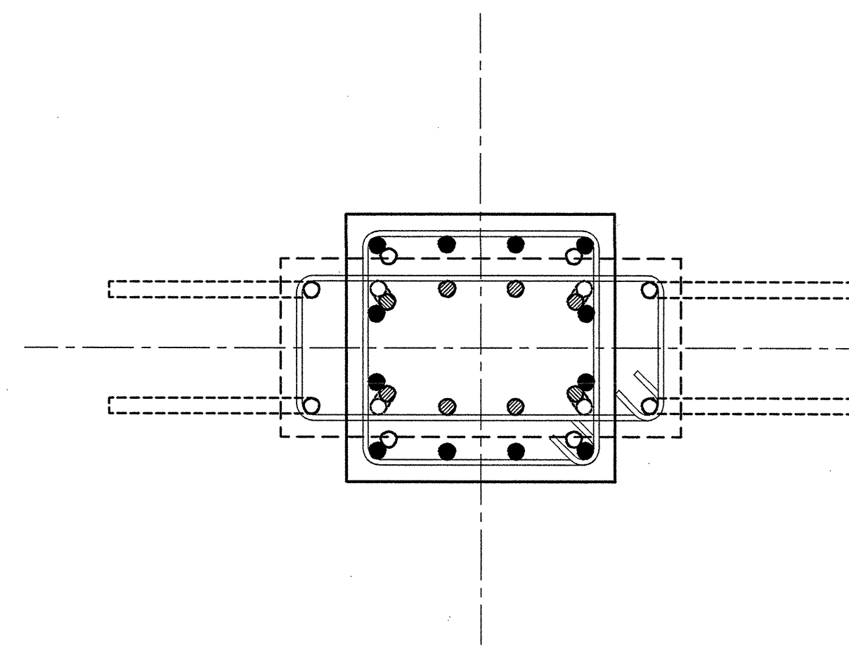
16"x36" TO 24"x24"
