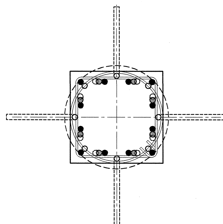
27"Ø TO 24"x24"
