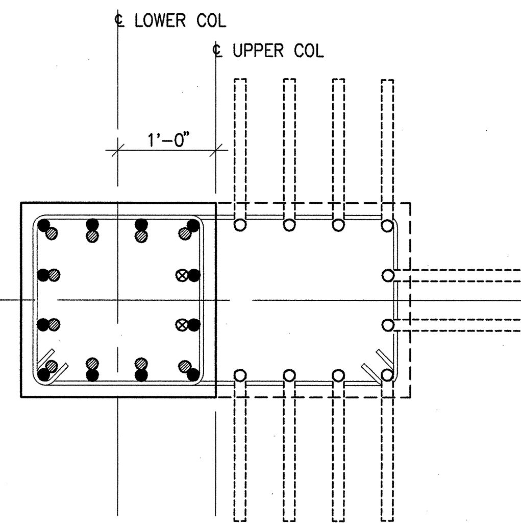
24"x48" TO 24"x24" W/ 12" OFFSET
