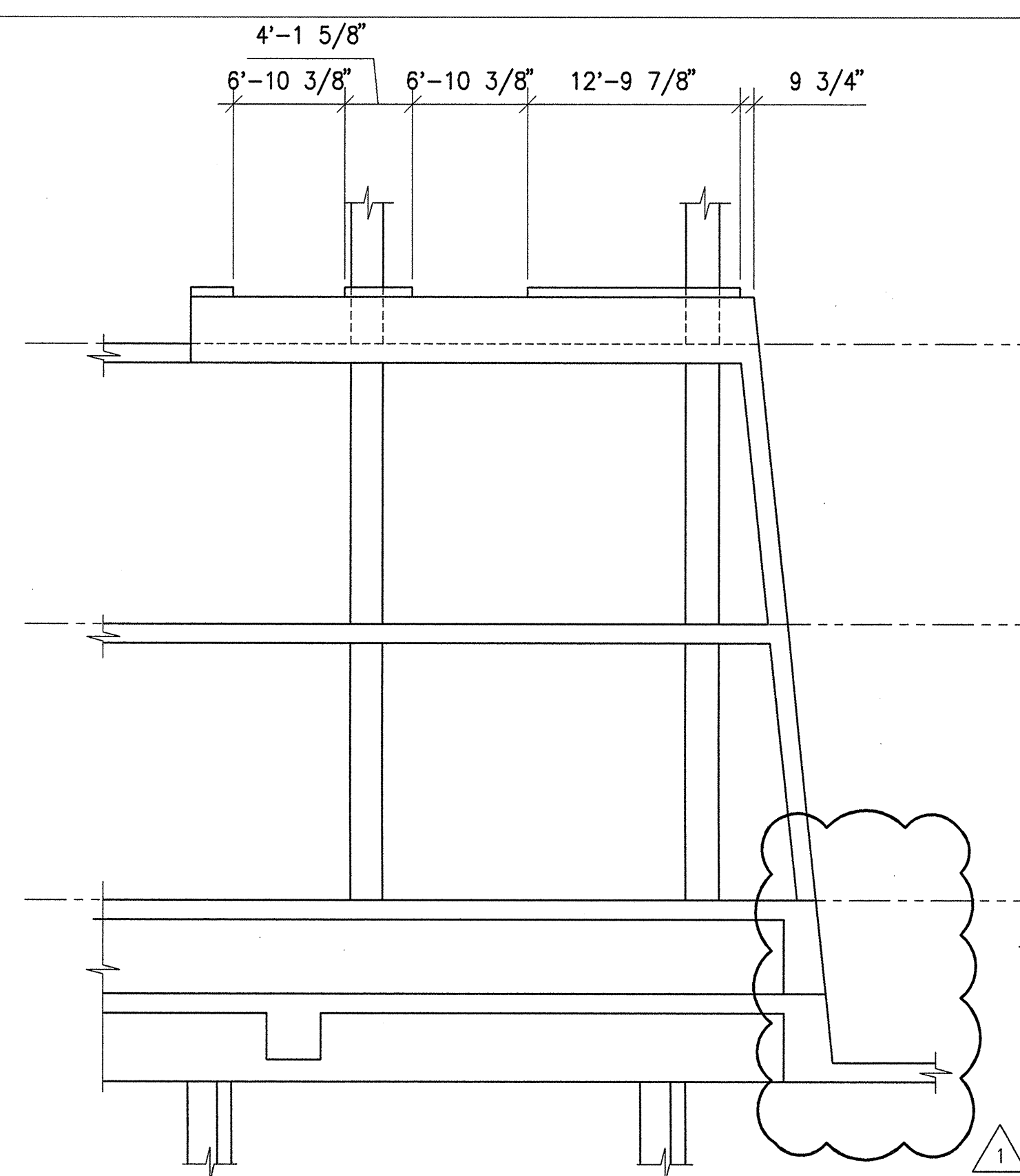
2C SOUTH WALL ELEVATION
