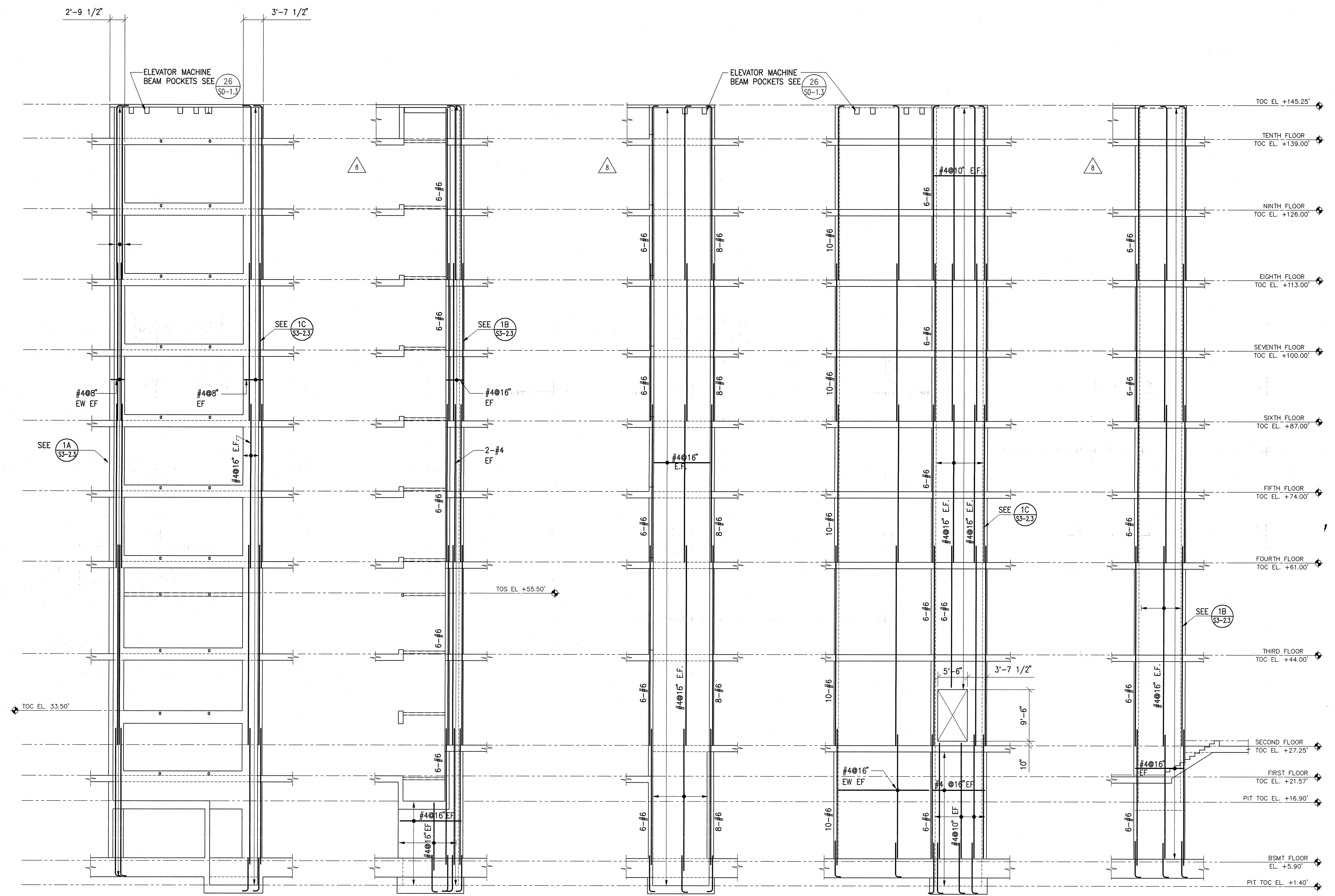
1E WEST WALL ELEVATION (THK = 10')
