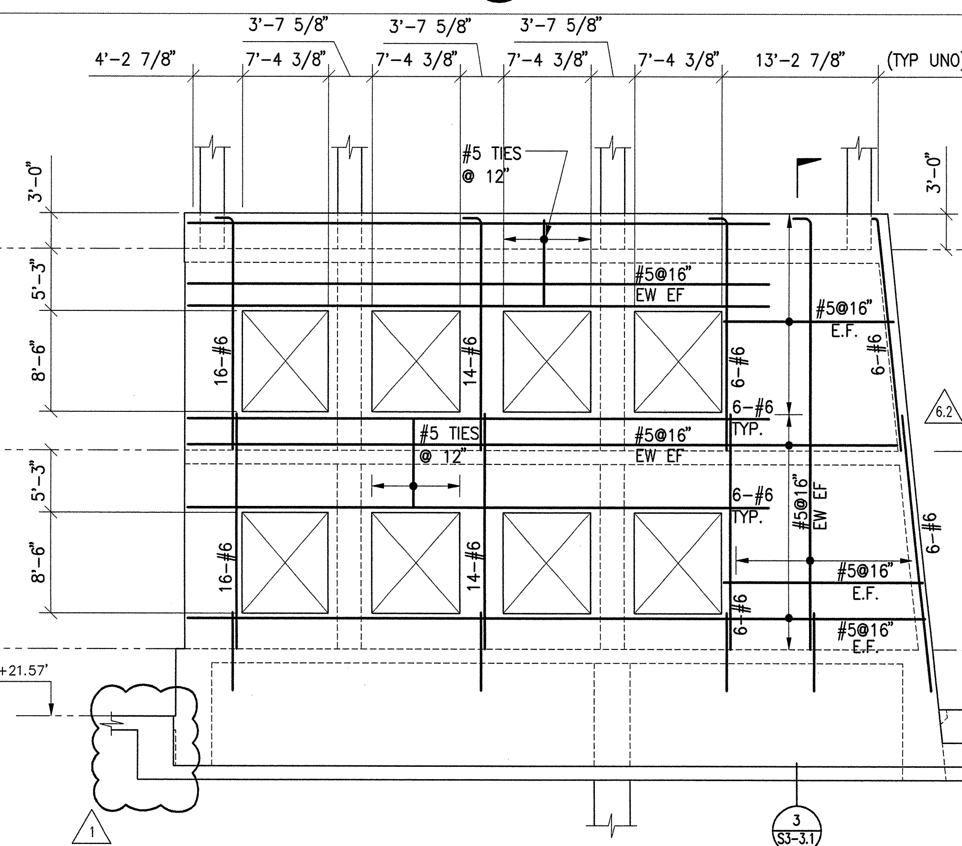
2B PROJECTED EAST WALL ELEVATION (SLOPED) (THK = 14')
