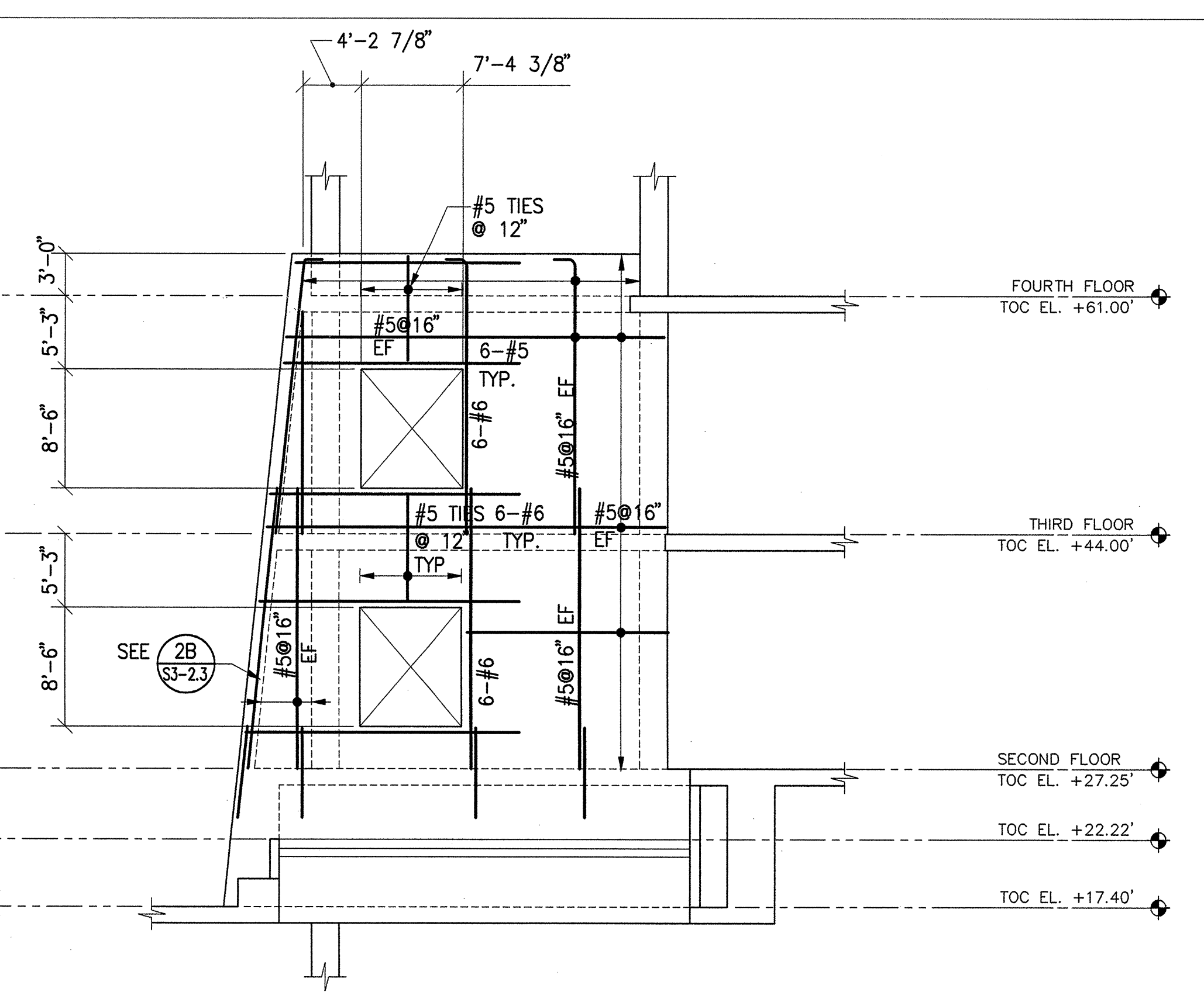
2A PROJECTED NORTH WALL ELEVATION (SLOPED)
