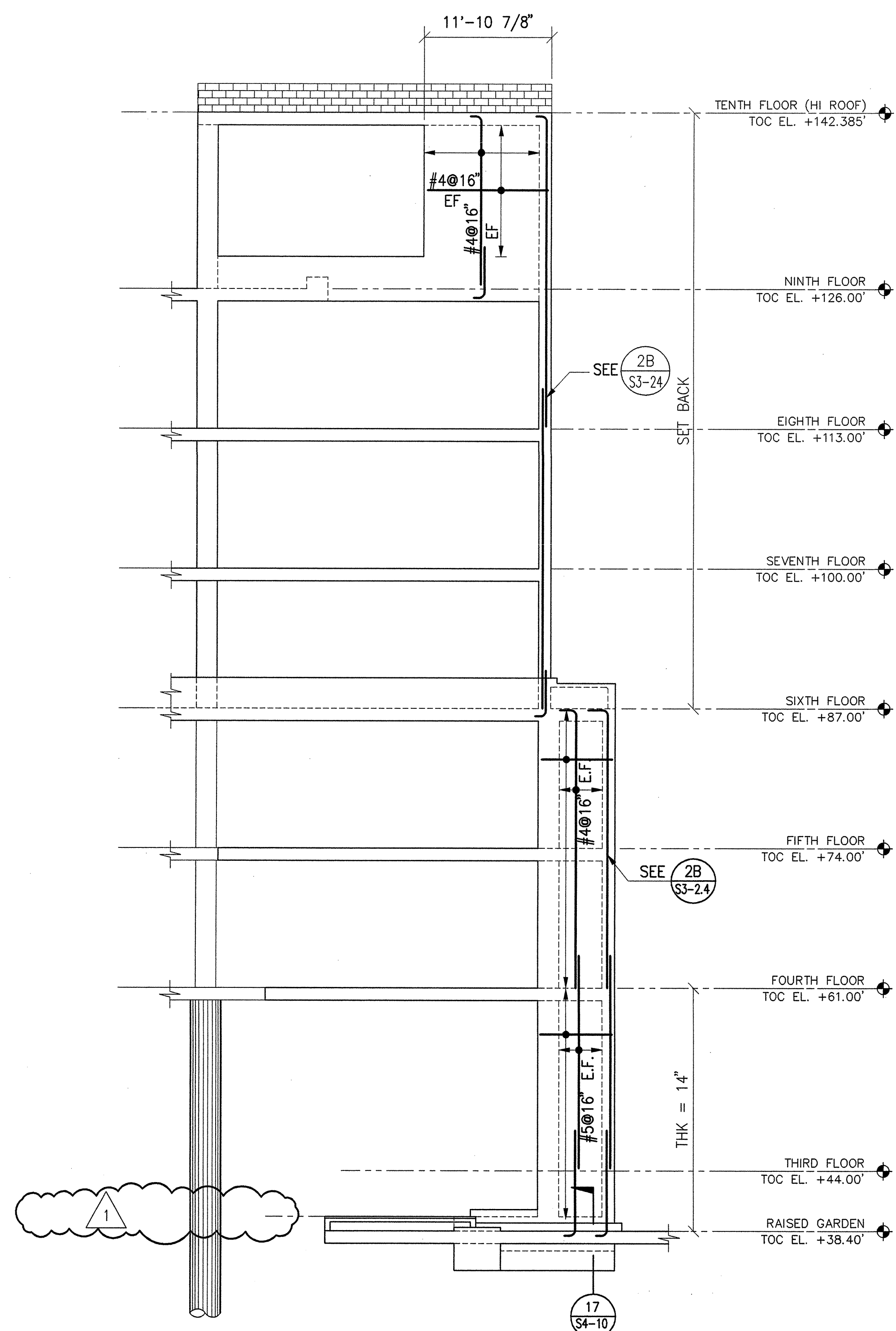
4 GATES SOUTH - WEST WALL ELEVATION 1/8"=1'-0" (THK = 10' UNO)
