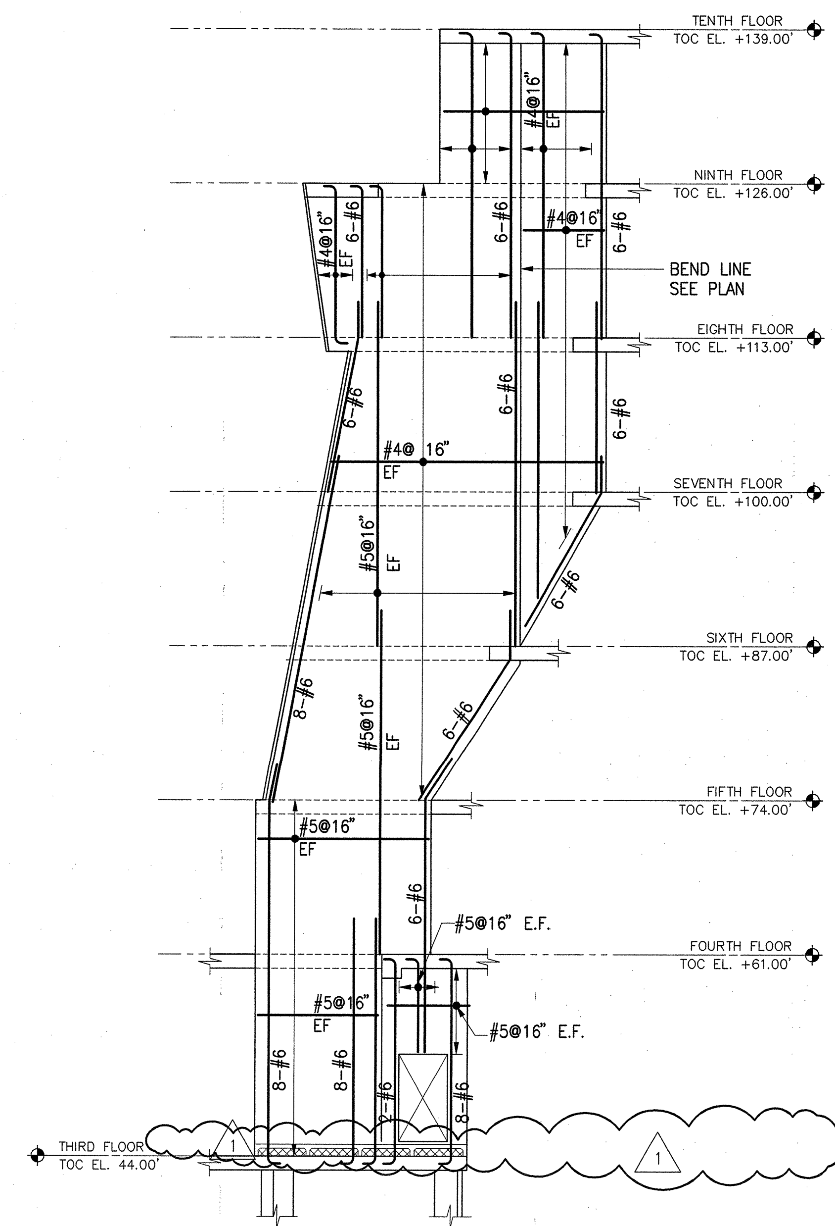
3 STAIR 4 - WEST WALL ELEVATION 1/8"=1'-0" (THK = 10')
