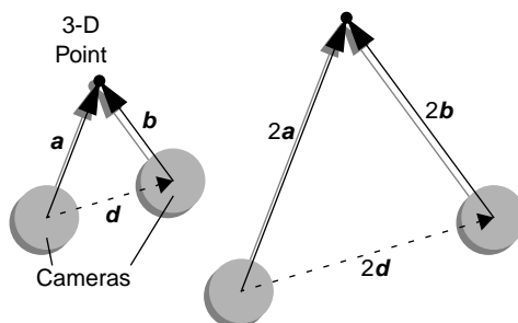
Figure 7: Scale Ambiguity
