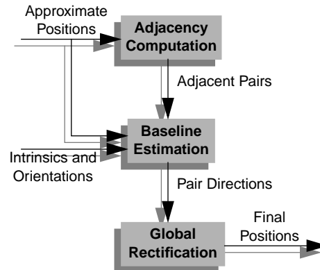
Figure 2: Translation Estimation
