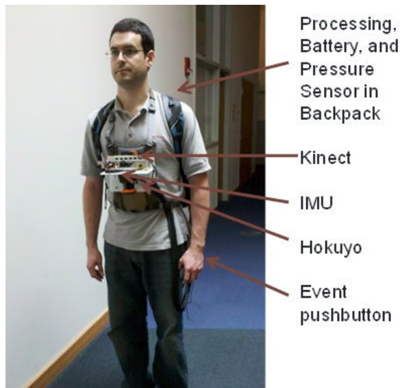
Fig. 1. A user carrying our prototype human-portable mapping system
