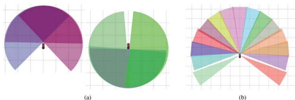
Figure 11. Sensor FOVs on 20-m grid. (a) Our vehicle used a total of seven horizontally mounted 180-deg planar LIDARs with overlapping FOVs. Front and rear LIDARs have been drawn separately to make the overlap more obvious. For ground plane rejection two LIDARs were required to “see” the same obstacle to register the detection (except in the very near field). (b) Fifteen radars with 18-deg FOV each were fanned to yield a wide (255-deg) total FOV.
