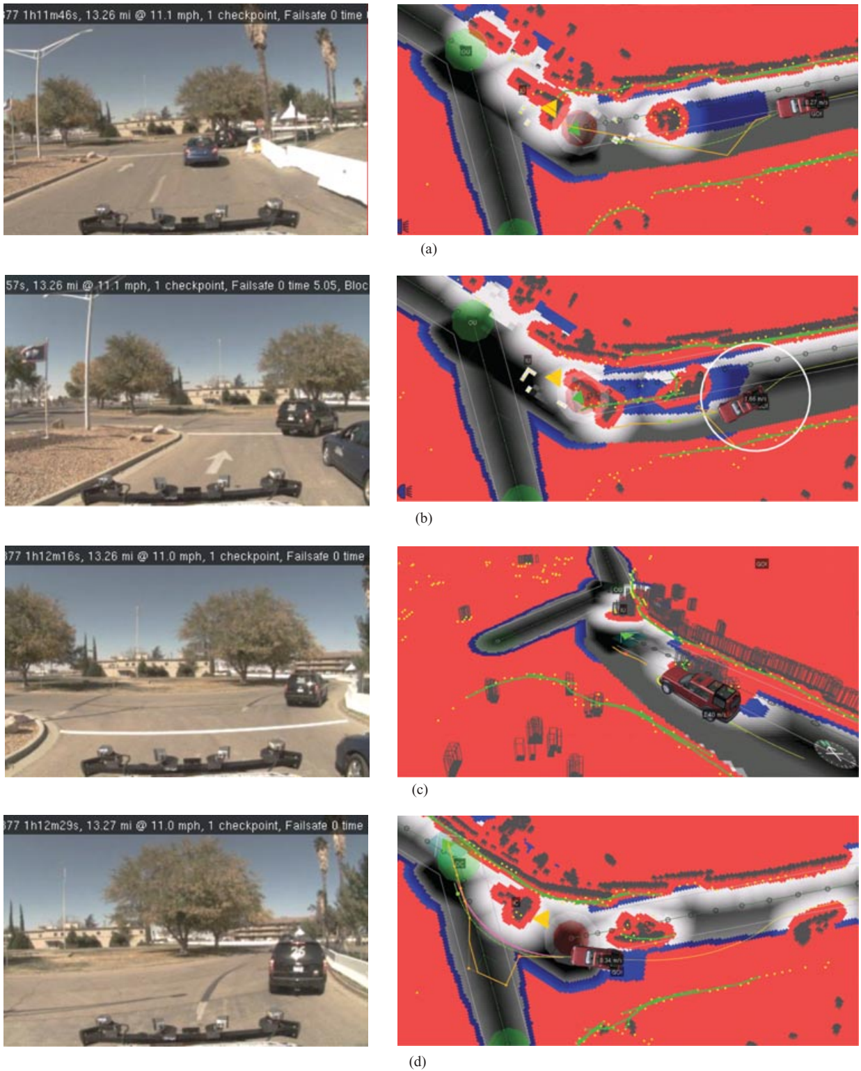
Figure 24. Lead-up to the Skynet–Talos incident. (a) Talos found a route around the chase vehicle. (b) Skynet backed up onto Talos’s goal position; Talos braked. (c) Skynet advanced again. Talos passed the chase vehicle. (d) Talos yielded at the intersection. There were no moving vehicles nearby, so it proceeded.
