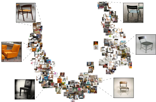
Fig. 11: Object graph visualization based on learned object representations: we visualize images using t-SNE [27] on predicted 3D viewpoint by 3D-INN.
