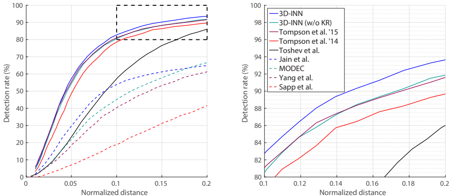
Fig. 4: PCK curves on the FLIC dataset. 3D-INN performs consistently better than other methods. Without keypoint refinement, it is comparable to Tompson et al. [43]. A zoomed view of the dashed rectangle is shown on the right.
