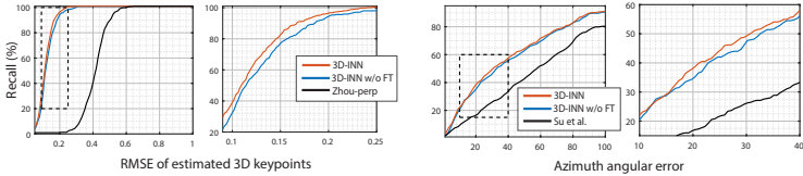
Fig. 6: Plots comparing our method against an analytic solution on synthetic heatmap. (a) The accuracy of 3D structure estimation; (b) The accuracy of 3D viewpoint estimation.
