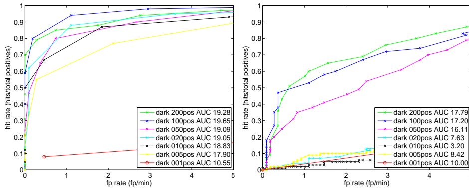
Figure 6: ``Wash`` ROC curves from our approach (left) versus the HMM-MFCC approach (right), for various numbers of positive training exemplars.
