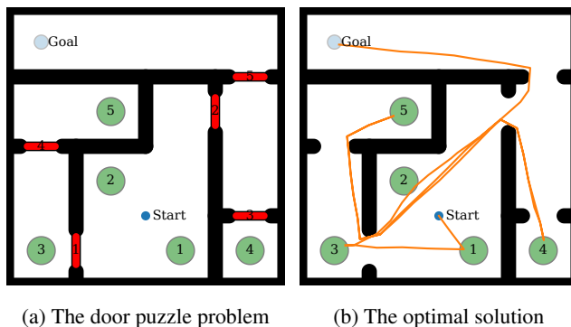
Figure 1: The door-switch problem, an example task and motion planning domain. A two-dimensional robot must navigate from the start location to a goal location, but the way is obstructed by doors that can only be opened by toggling a corresponding switch. The optimal solution to this problem instance is to toggle the switches in the order (1, 3, 2, 4, 5) and then go to the goal set. Because the size of the configuration space grows exponentially with the number of doors, planning is computationally challenging. Abstraction can render such planning problems tractable.
