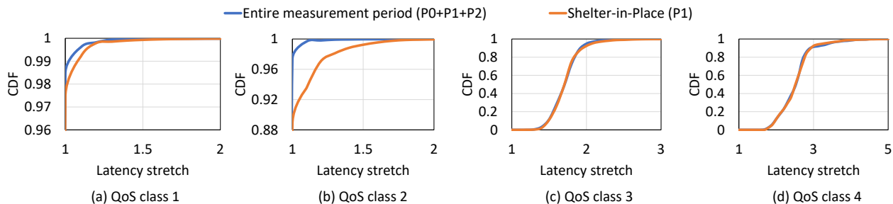
Figure 6: CDF of per-flow latency stretch for each QoS class.
