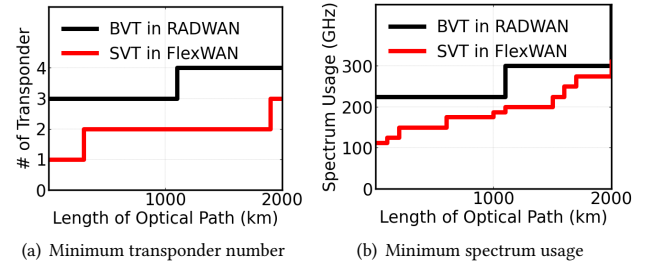
Figure 3: A typical example of hardware costs for provisioning 800 Gbps WAN capacity at different optical path lengths.
