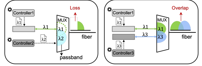
(a) Channel inconsistency
