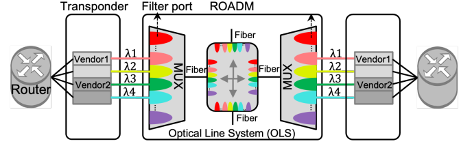
Figure 1: Overview of the fixed optical backbones.
